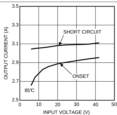
Figure 30. Current Limit, V_{OUT} = 3.3\text{ V} , T_A = 85^\circ\text{C}
