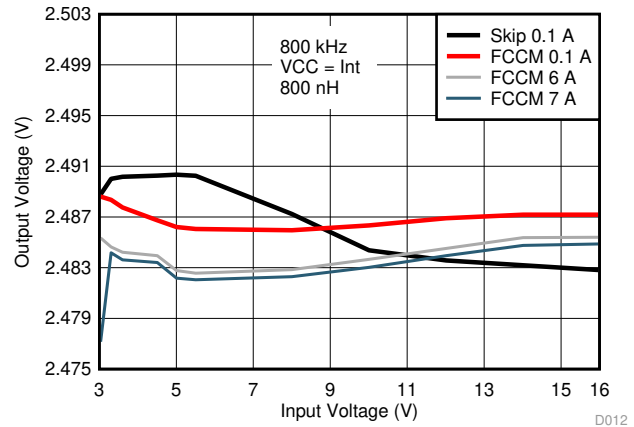
Figure 31. Output Voltage vs Input Voltage VCC = Int
