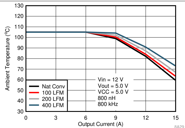
Figure 6. Safe Operating Area, V_{OUT} = 5 V
