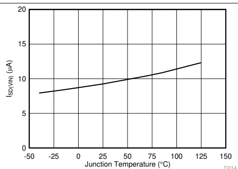
Figure 8. I_{SD(V_{IN})} vs Junction Temperature
