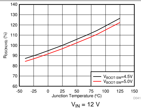
Figure 13. R_{DS(on)(HS)} vs Junction Temperature
