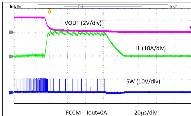
Figure 51. Overcurrent Protection
