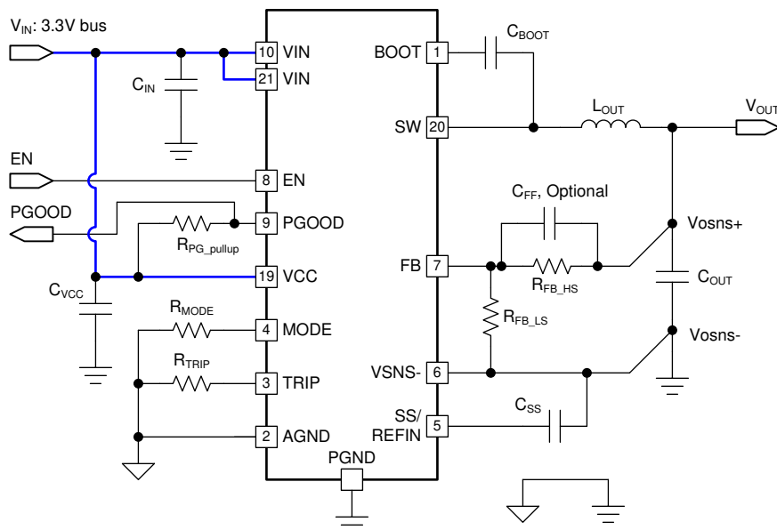
Figure 19. Single VIN Configuration With 3.3-V Bus
