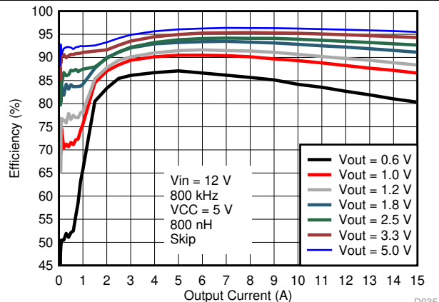
Figure 23. Efficiency vs Output Current, VCC = 5.0V External VCC Bias
