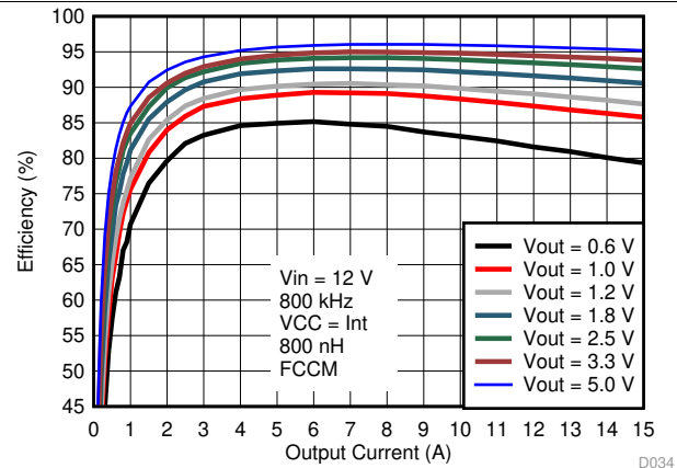
Figure 2. Efficiency vs Output Current, FCCM, Internal VCC LDO
