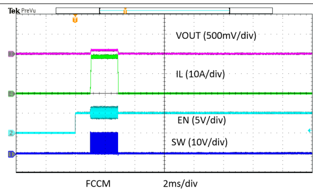
Figure 52. Enabled into Overcurrent
