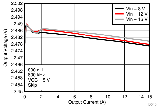
Figure 29. Output Voltage vs Output Current, VCC = 5.0V External Bias
