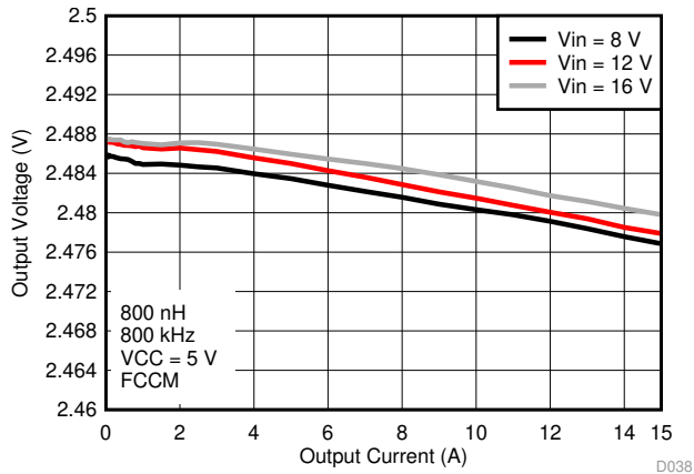
Figure 30. Output Voltage vs Output Current, VCC = 5.0V External Bias
