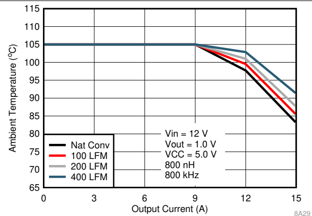
Figure 4. Safe Operating Area, V_{OUT} = 1.0 V
