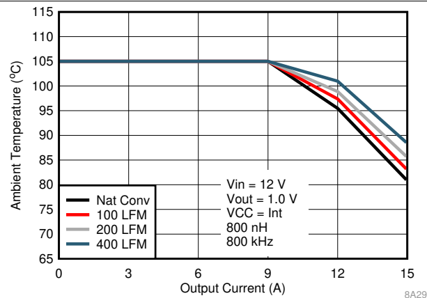
Figure 3. Safe Operating Area, V_{OUT} = 1.0 V
