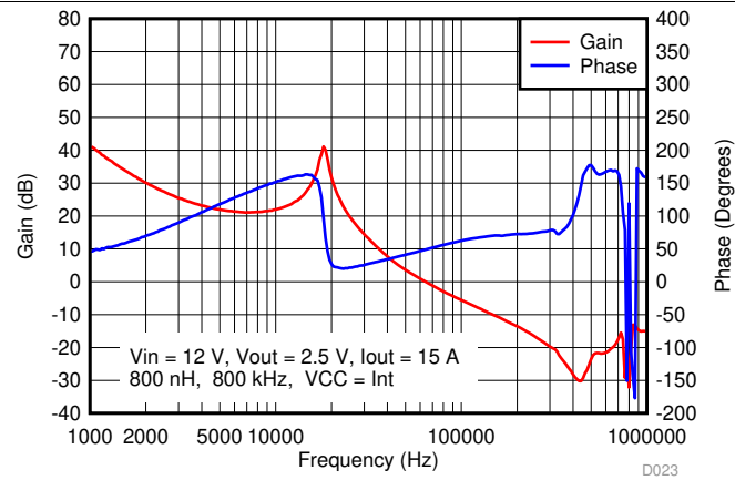
Figure 53. Frequency Response, 15 A Load
