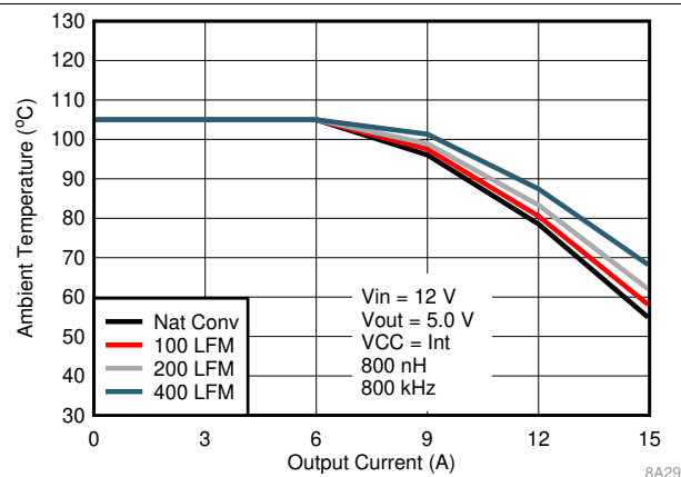
Figure 5. Safe Operating Area, V_{OUT} = 5 V
