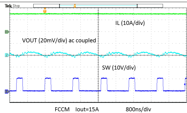
Figure 48. Output Voltage Ripple
