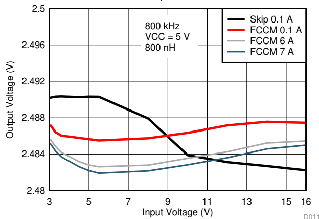
Figure 32. Output Voltage vs Input Voltage VCC = 5.0V External Bias
