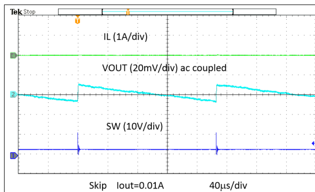
Figure 49. Output Voltage Ripple, Skip
