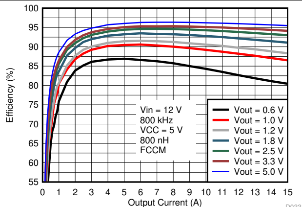
Figure 22. Efficiency vs Output Current, VCC = 5.0V External VCC Bias
