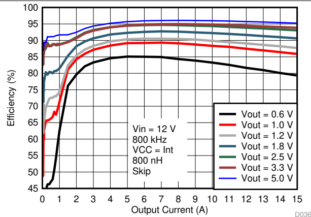
Figure 1. Efficiency vs Output Current, Skip-mode, Internal VCC LDO
