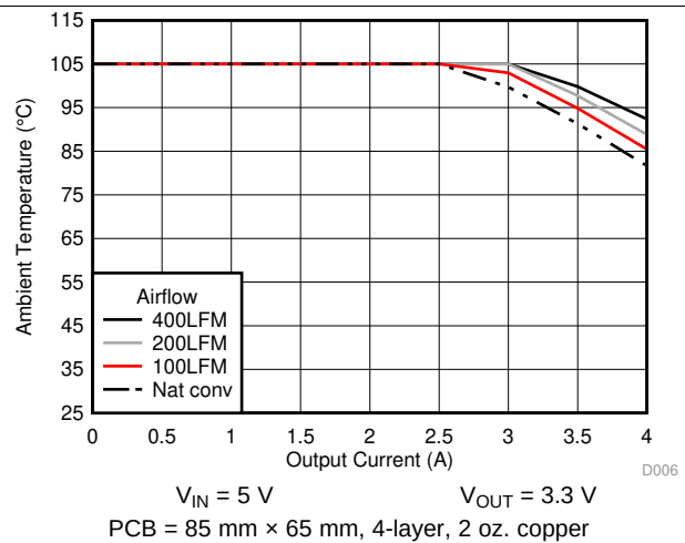
图 6. Safe Operating Area
