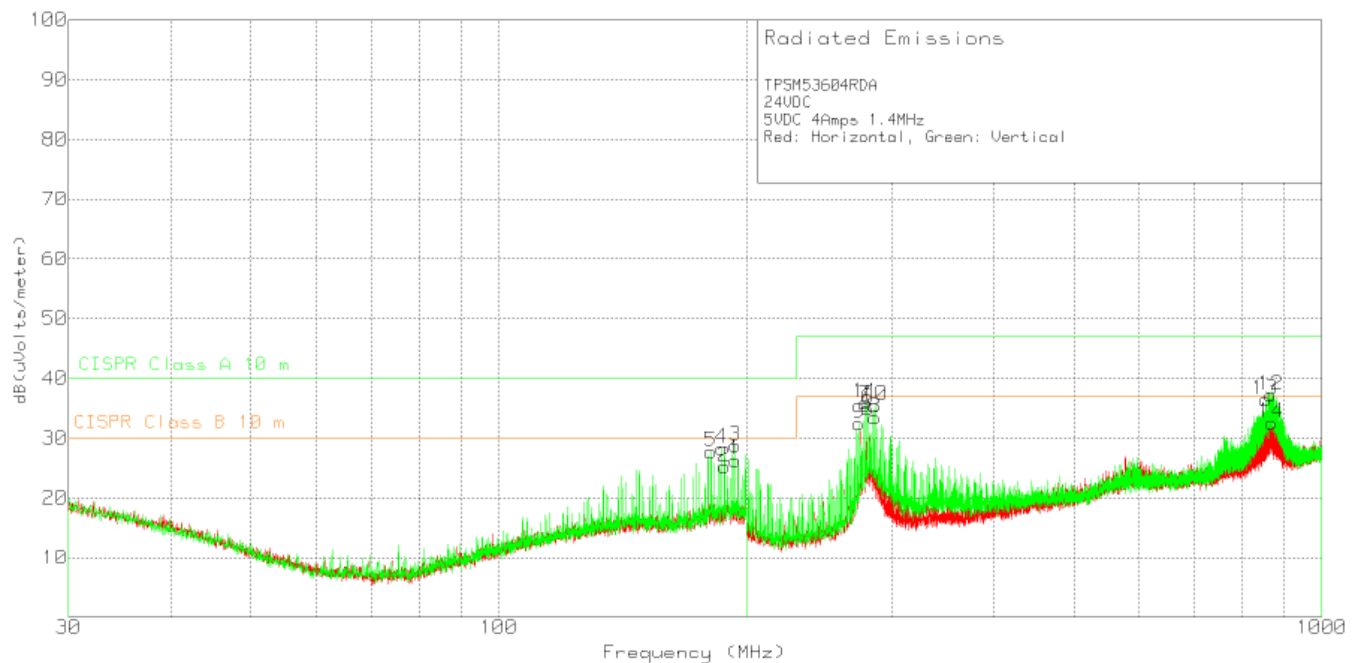
图 48. Radiated Emissions 24-V Input, 5-V Output, 4-A Load
