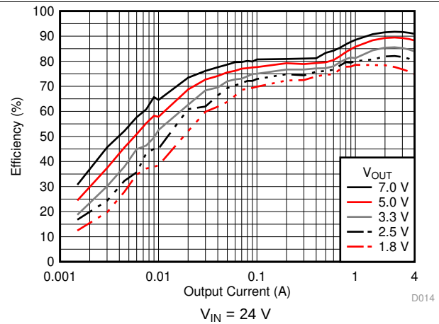
图 14. Efficiency versus Output Current
