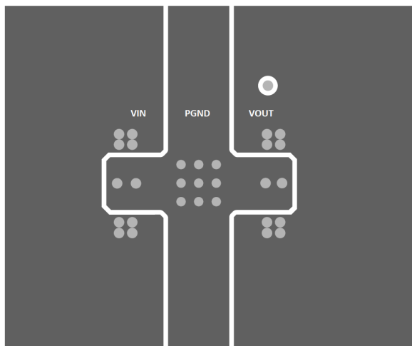
图 45. Typical Layer-2 Layout
