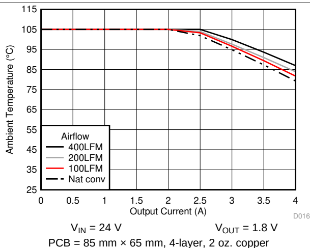
图 17. Safe Operating Area
