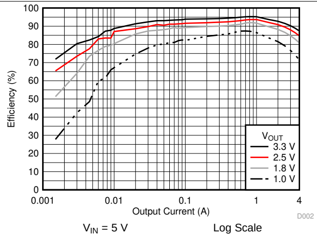
图 2. Efficiency versus Output Current
