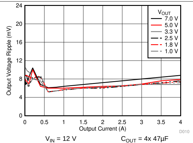
图 10. Voltage Ripple versus Output Current
