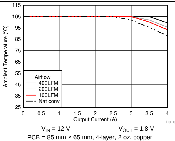
图 11. Safe Operating Area
