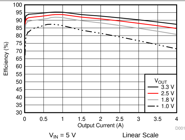
图 1. Efficiency versus Output Current
