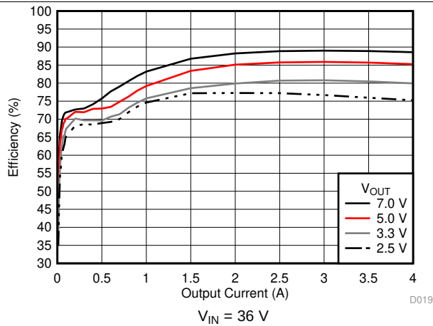
图 19. Efficiency versus Output Current
