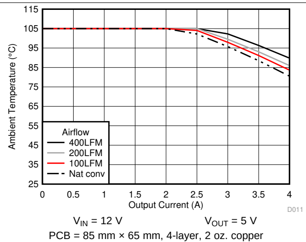
图 12. Safe Operating Area
