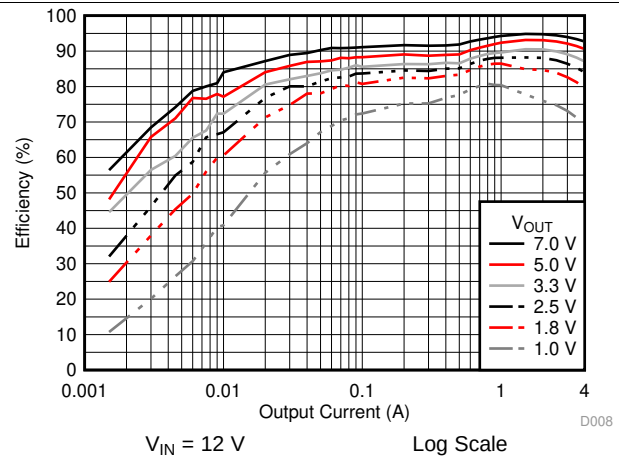
图 8. Efficiency versus Output Current
