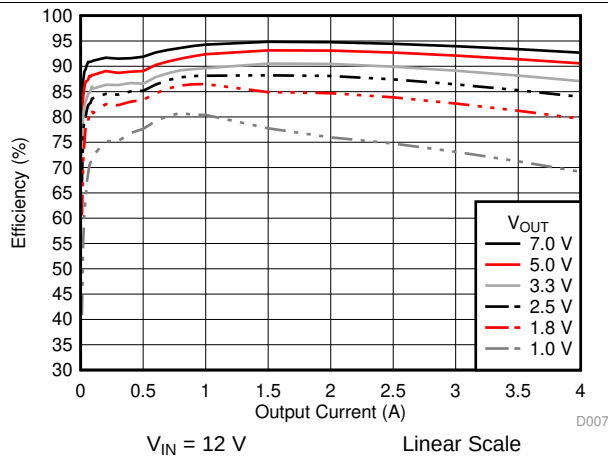
图 7. Efficiency versus Output Current
