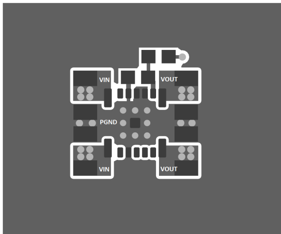
图 44. Typical Top-Layer Layout
