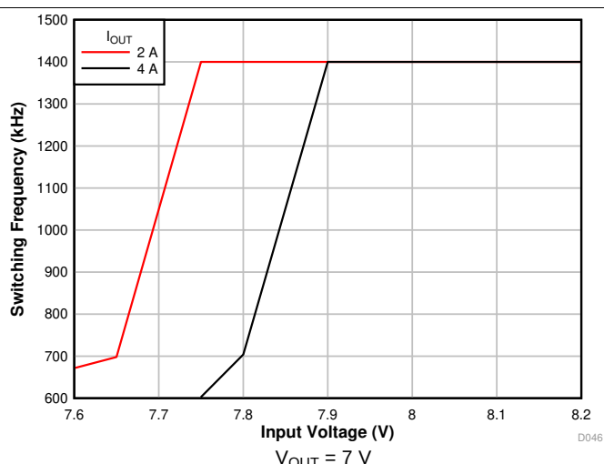
图 36. Frequency Foldback
