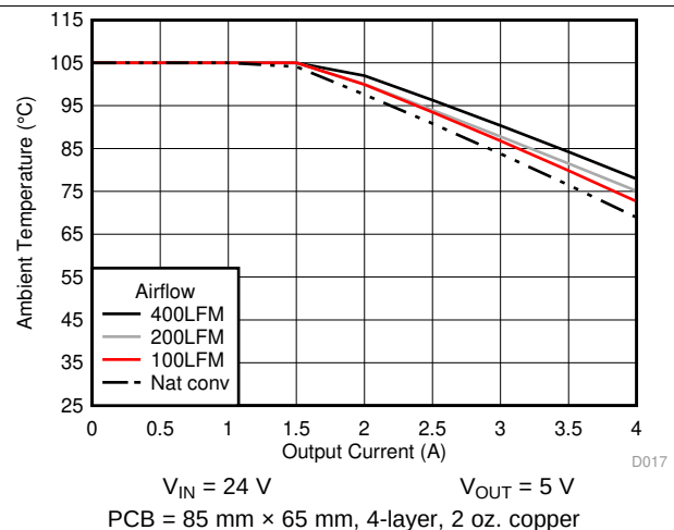
图 18. Safe Operating Area
