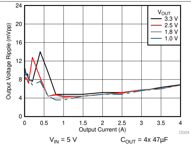
图 4. Voltage Ripple versus Output Current
