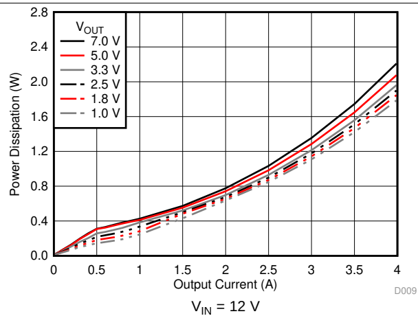
图 9. Power Dissipation versus Output Current
