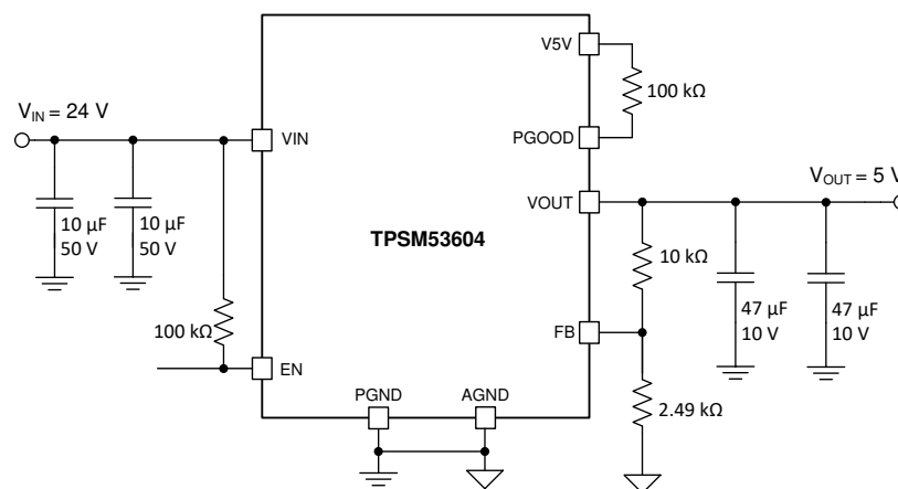
图 40. TPSM53604 Typical Schematic
