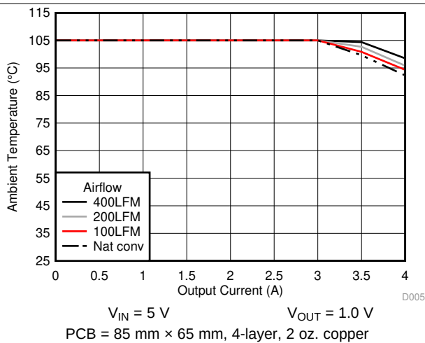
图 5. Safe Operating Area
