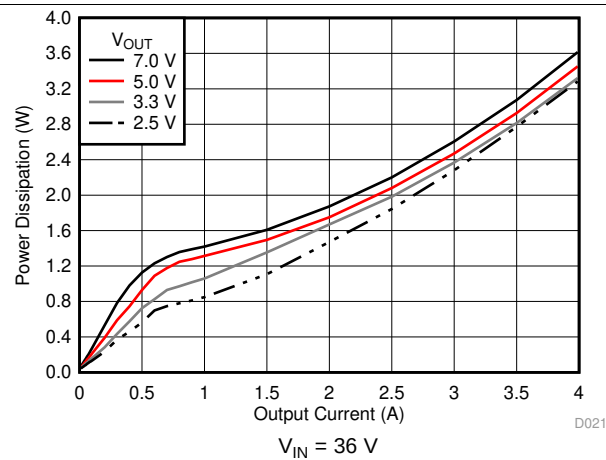
图 21. Power Dissipation versus Output Current
