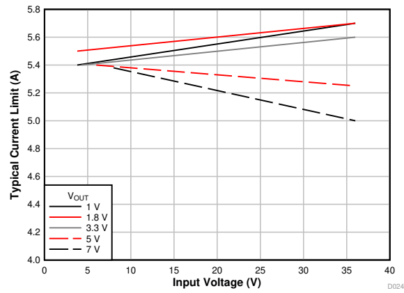
图 37. Current Limit Threshold
