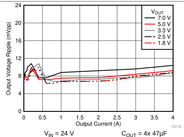
图 16. Voltage Ripple versus Output Current
