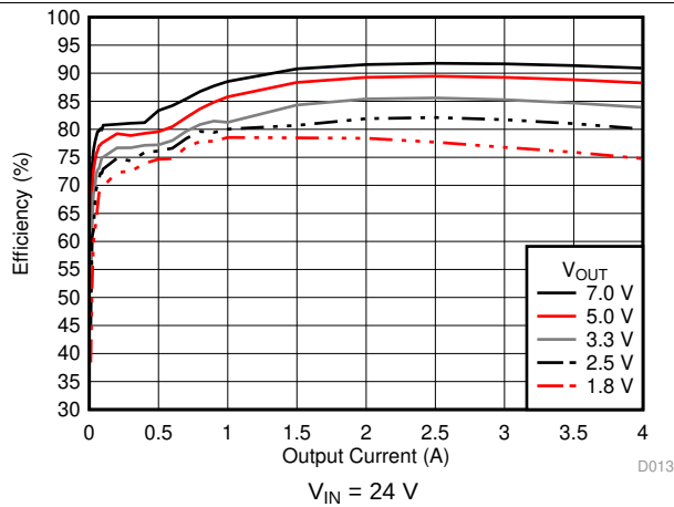
图 13. Efficiency versus Output Current
