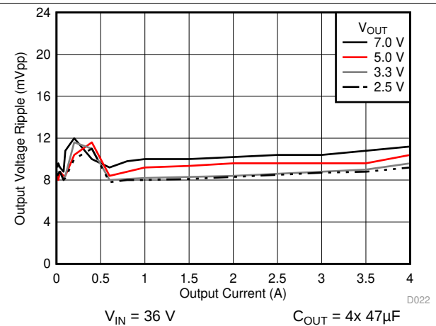
图 22. Voltage Ripple versus Output Current
