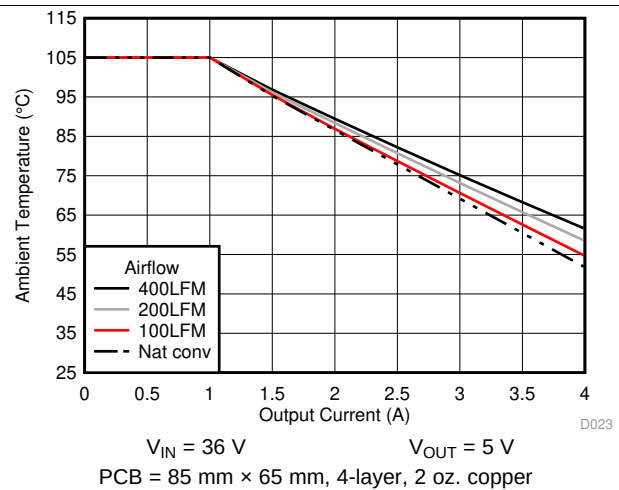
图 24. Safe Operating Area
