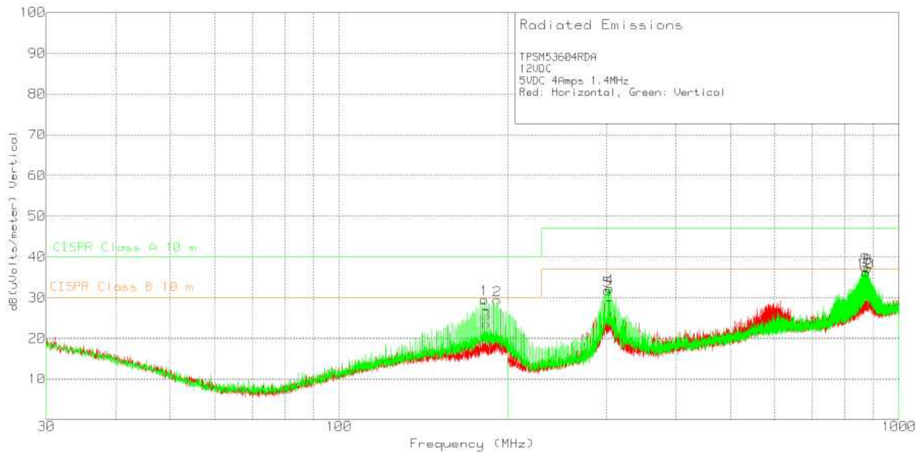
图 49. Radiated Emissions 12-V Input, 5-V Output, 4-A Load
