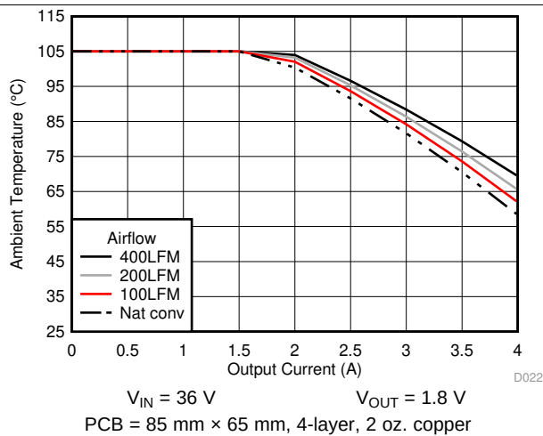
图 23. Safe Operating Area
