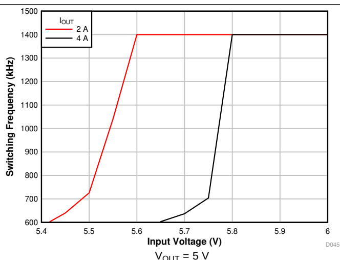
图 34. Frequency Foldback
