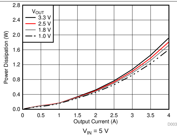
图 3. Power Dissipation versus Output Current
