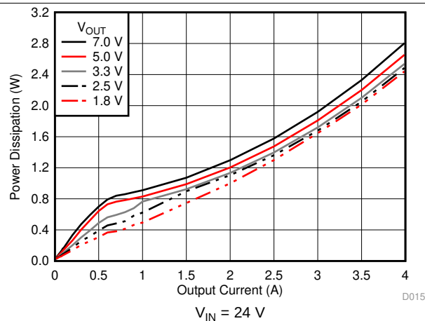
图 15. Power Dissipation versus Output Current
