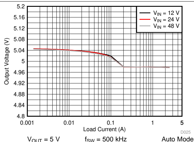
图 49. LM76002-Q1 Load and Line Regulation
