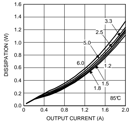
Figure 20. Dissipation 8-V Input at 85°C
