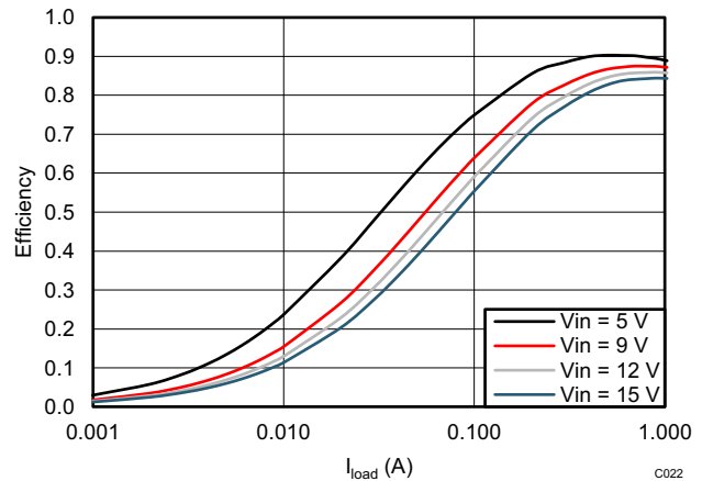
图 6-16. TPS562208 V_{OUT} = 1.8\text{ V} Efficiency, L = 2.2\text{ }\mu\text{H}
