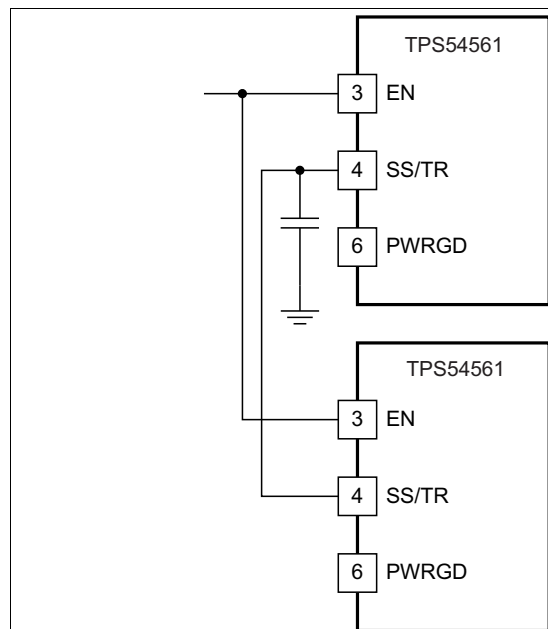
Figure 31. Schematic for Ratio-Metric Start-Up Sequence
