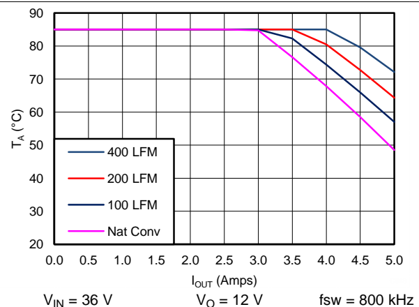
Figure 50. Air Flow Conditions
