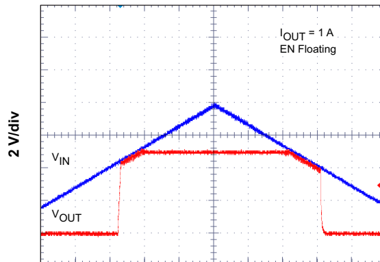
Figure 62. Low Dropout Operation
