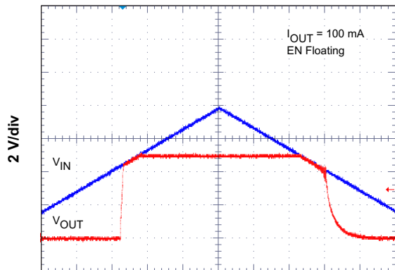
Figure 61. Low Dropout Operation
