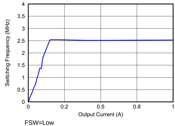
Figure 23. Switching Frequency
