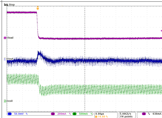
Figure 29. Load Transient Response ( I_{OUT} = 0.5\text{ to }1\text{ to }0.5\text{ A} , V_{IN} = 12\text{ V} , V_{OUT} = 3.3\text{ V} )
