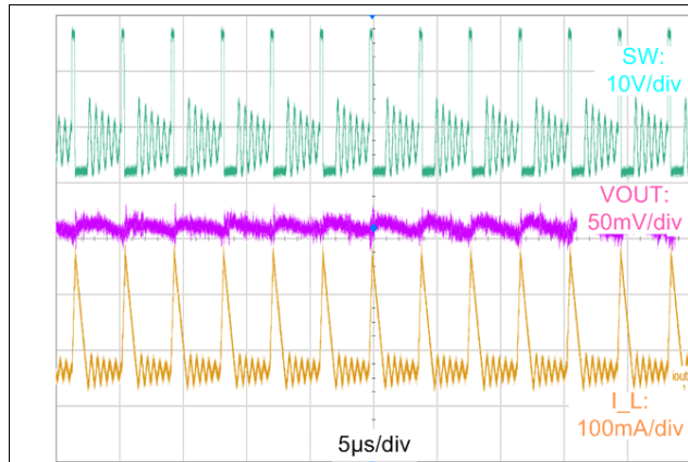
图 13. Typical PFM Switching Waveforms V_{IN} = 24\text{ V} , V_{OUT} = 5\text{ V} , I_{OUT} = 30\text{ mA}
