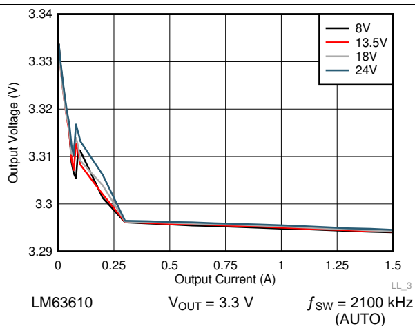
Figure 25. Line and Load Regulation
