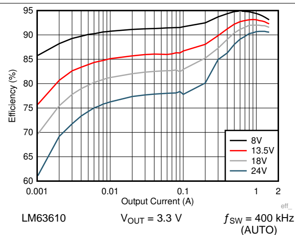
Figure 22. Efficiency
