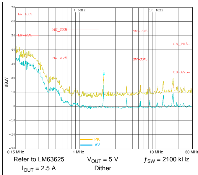
Figure 39. Typical Conducted EMI with LM63625 0.15 MHz to 30 MHz
