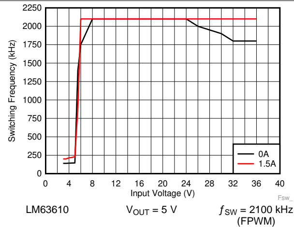
Figure 28. Switching Frequency versus Input Voltage
