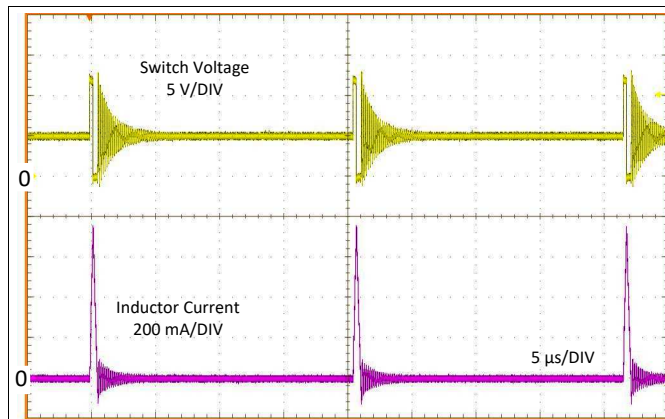
Figure 8. Typical PFM Switching Waveforms V_{IN} = 12\text{ V} , V_{OUT} = 5\text{ V} , I_{OUT} = 10\text{ mA}
