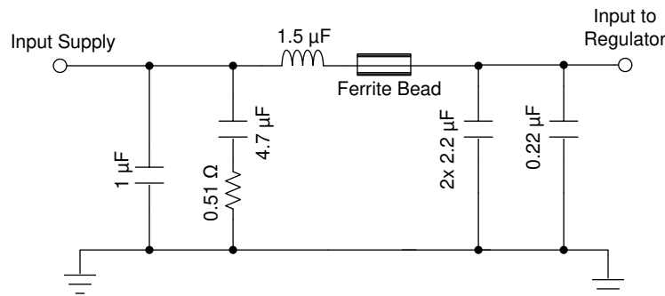
Figure 41. Typical Input EMI Filter with LM63625
