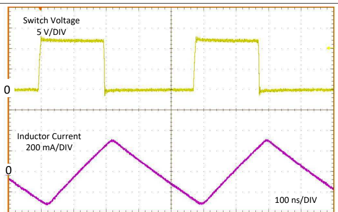
Figure 9. Typical PWM Switching Waveforms FPWM V_{IN} = 12\text{ V} , V_{OUT} = 5\text{ V} , I_{OUT} = 0\text{ A} , f_{SW} = 2100\text{ kHz}
