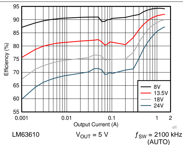
Figure 21. Efficiency
