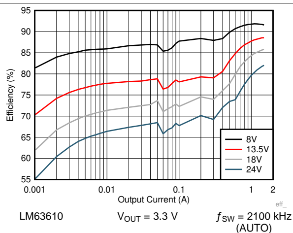
Figure 23. Efficiency
