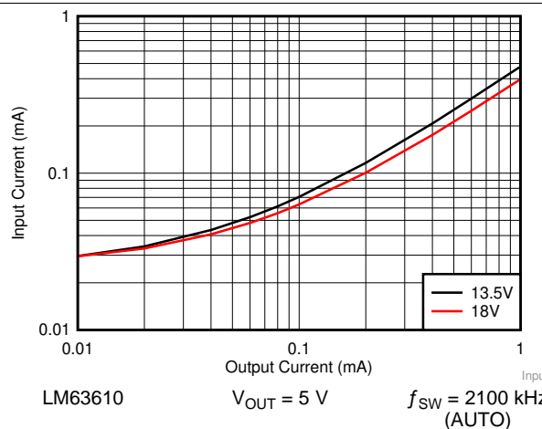
Figure 36. Input Supply Current versus Output Current
