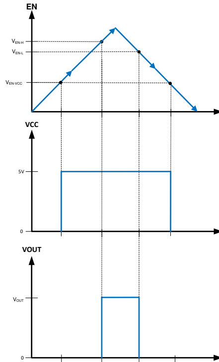
Figure 5. Precision Enable Behavior
