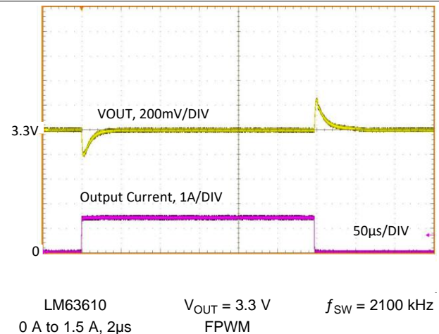
Figure 29. Load Transient
