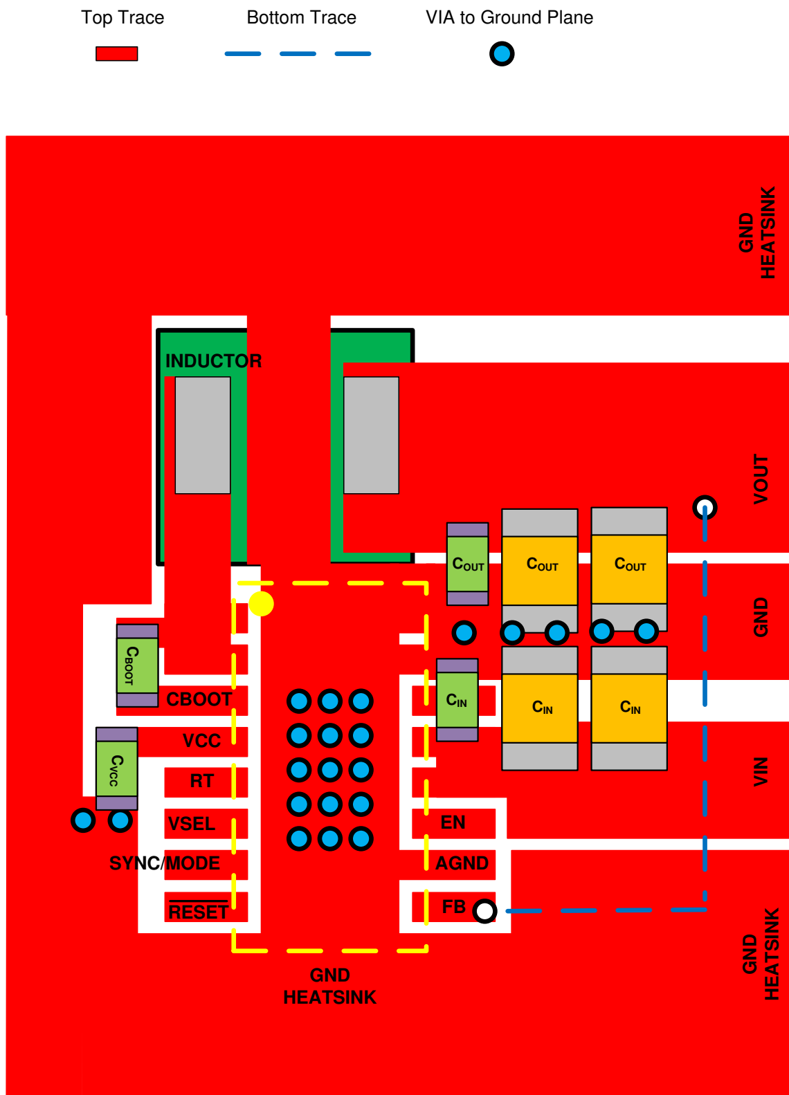
Figure 43. Example Layout
