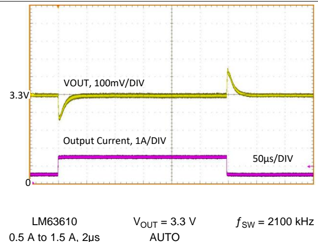
Figure 31. Load Transient
