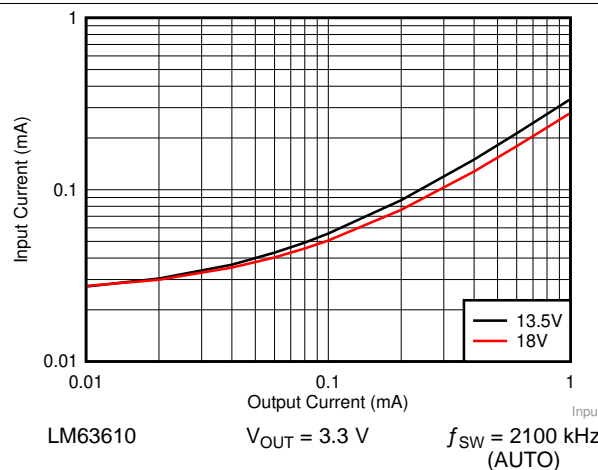
Figure 37. Input Supply Current versus Output Current
