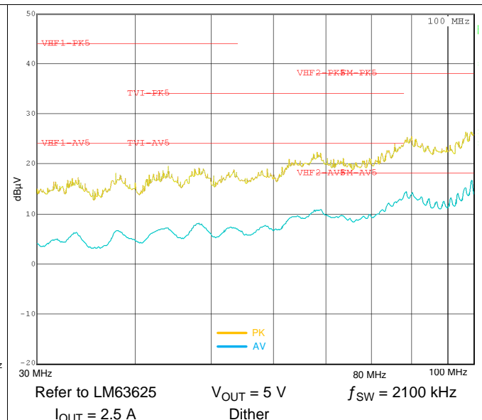
Figure 40. Typical Conducted EMI with LM63625 30 MHz to 108 MHz
