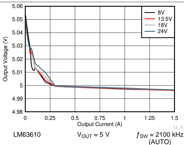
Figure 24. Line and Load Regulation
