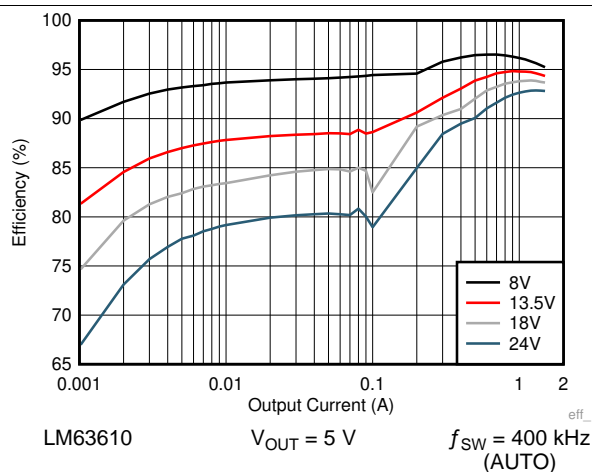
Figure 20. Efficiency
