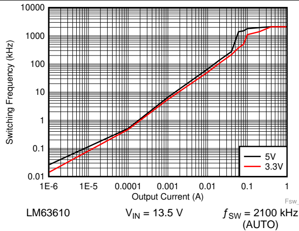
Figure 26. Switching Frequency versus Output Current
