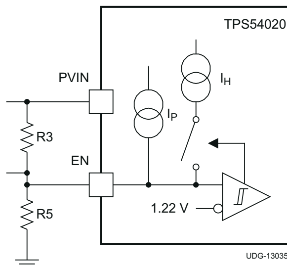
图 8-2. Adjustable PVIN Undervoltage Lockout, PVIN \geq 4.5 \text{ V}
