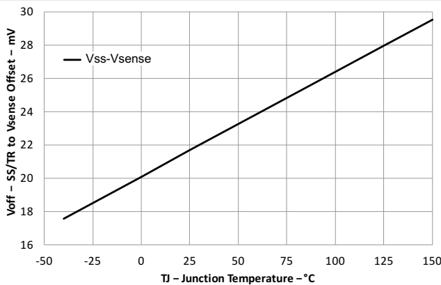
图 7-11. (V_{SS} - V_{VSENSE}) Offset vs Junction Temperature
