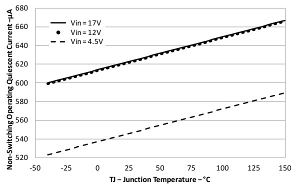
图 7-9. Nonswitching Operating Current vs Junction Temperature
