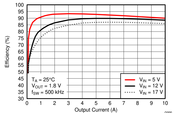
图 9-15. Efficiency
