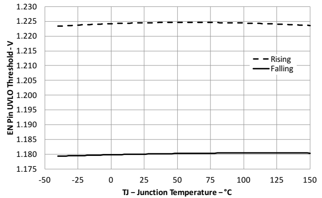
图 7-8. EN Pin UVLO Threshold vs Junction Temperature, V_{VIN} = 12\text{ V}
