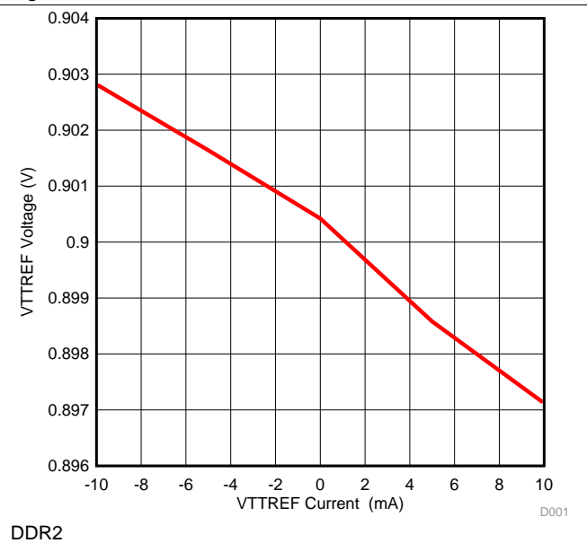
Figure 18. VTTREF Load Regulation
