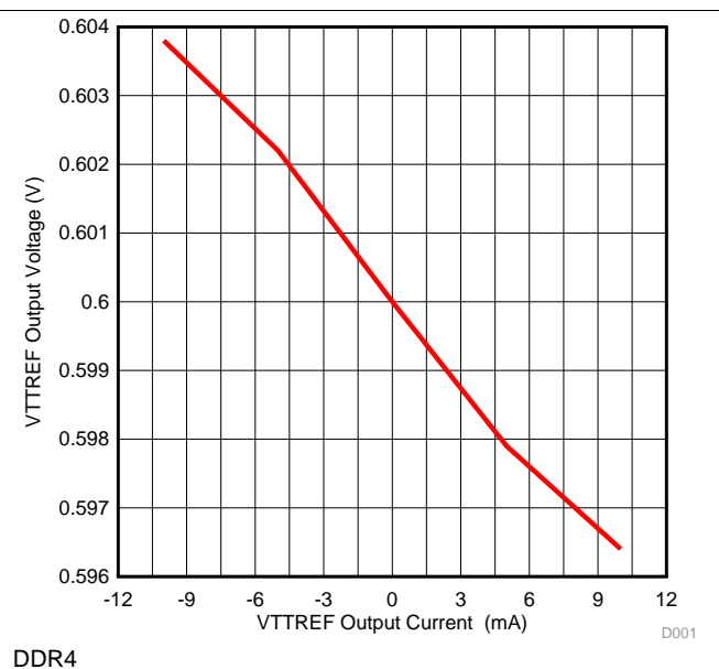
Figure 20. VTTREF Load Regulation
