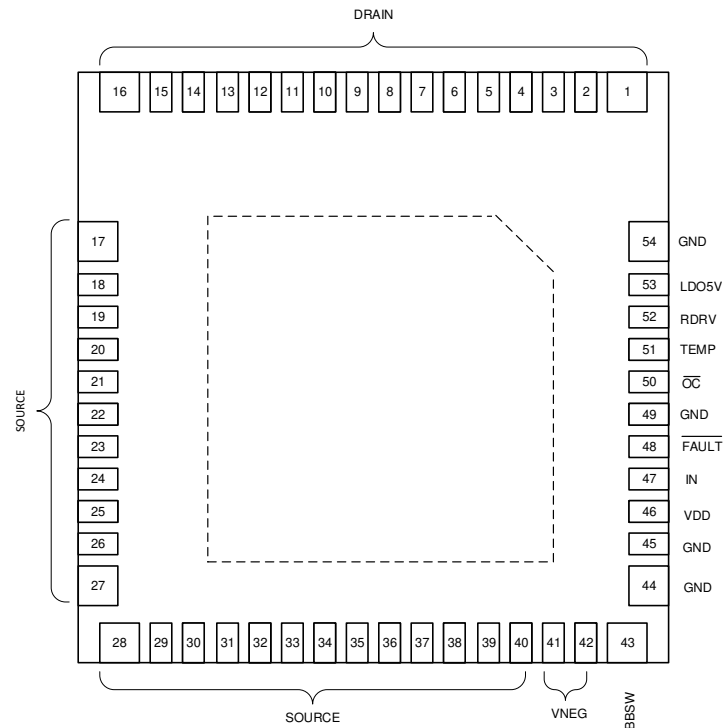
Figure 6-1. RQZ (VQFN) Package 54 Pins (Top View)
