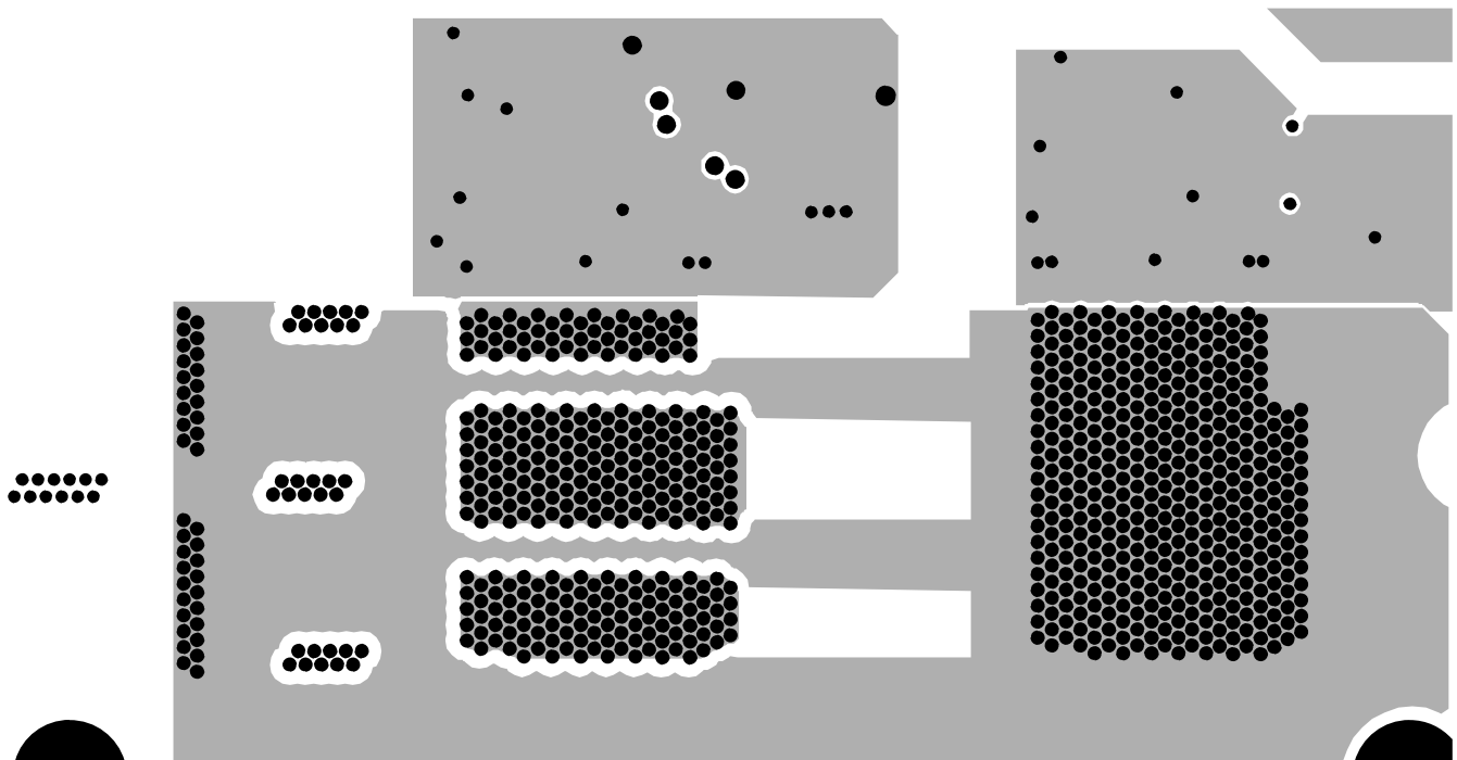
Figure 12-2. Half-Bridge Mid Layer Layout
