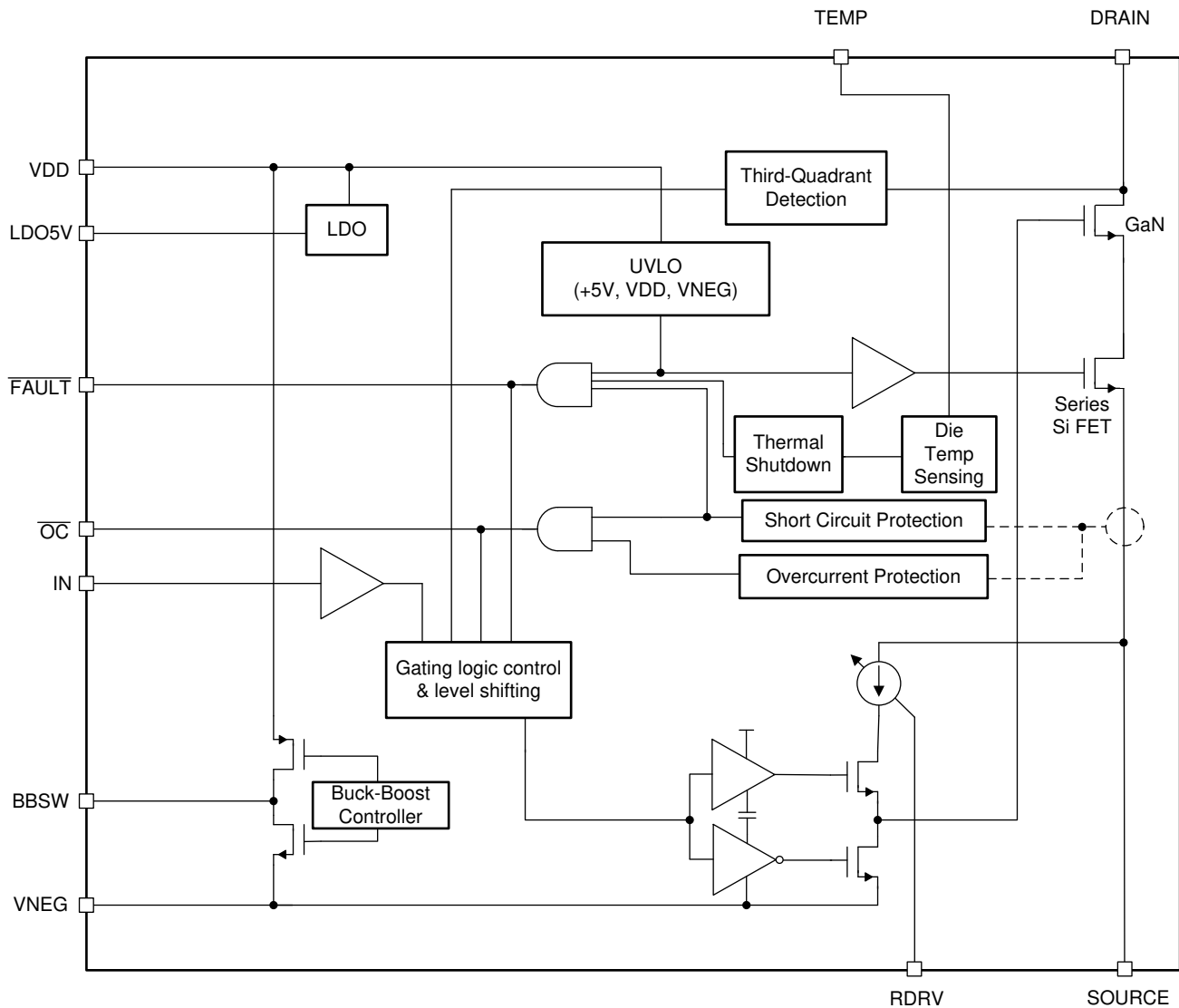
Figure 9-1. Simplified Block Diagram of LMG342xR030
