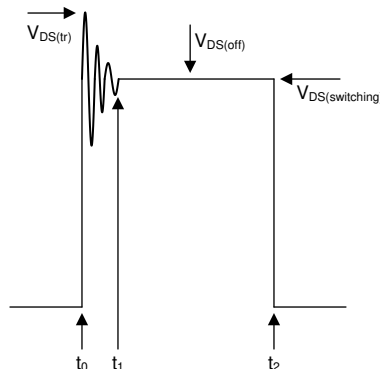
Figure 9-2. Drain-Source Voltage Switching Cycle
