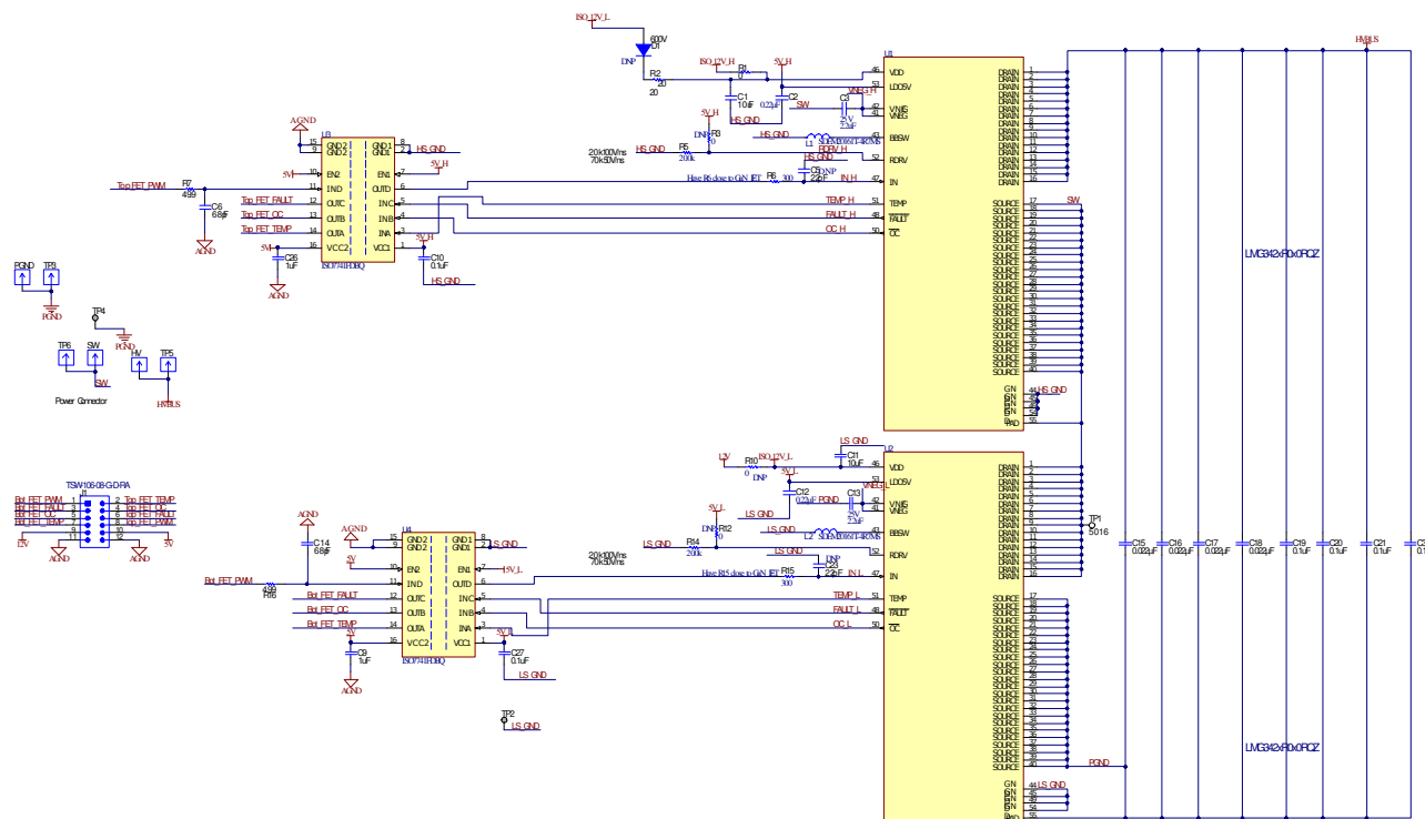
Figure 10-1. Typical Half-Bridge Application
