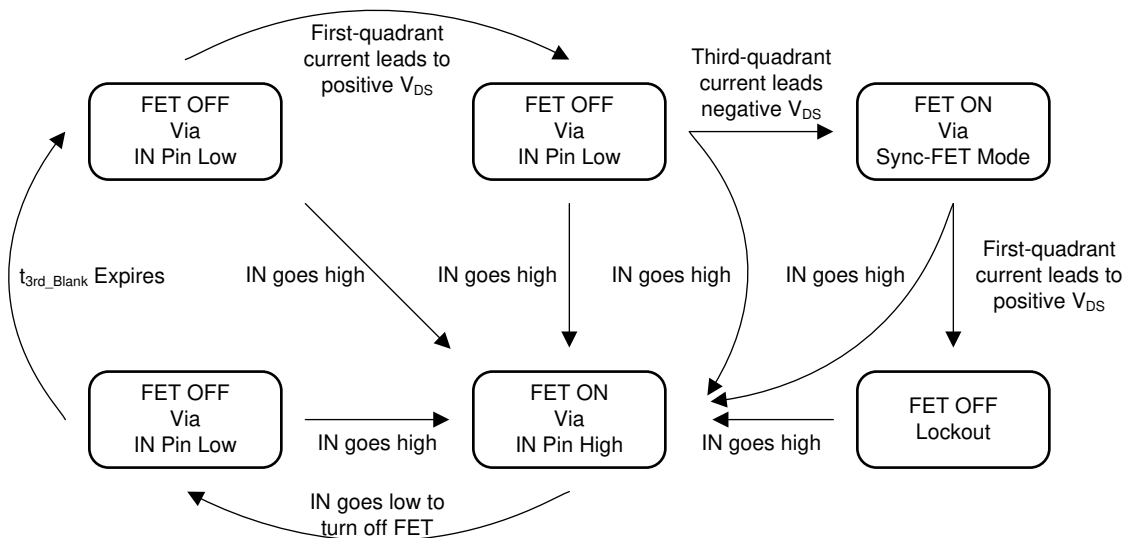
Figure 9-6. Sync FET Mode State Machine
