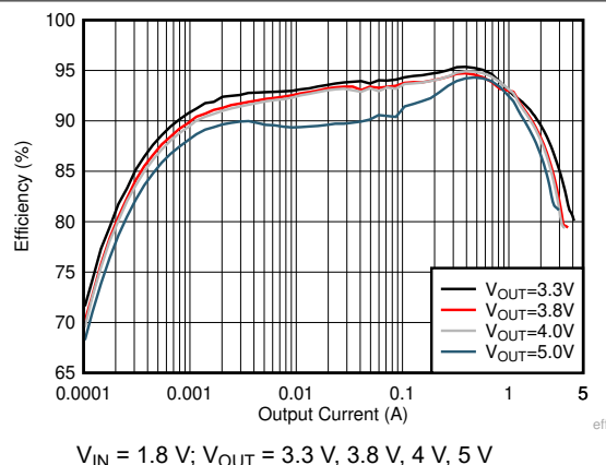
Figure 6-2. Load Efficiency With Different Output in Auto PFM
