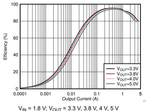
Figure 6-4. Load Efficiency With Different Output in Forced PWM
