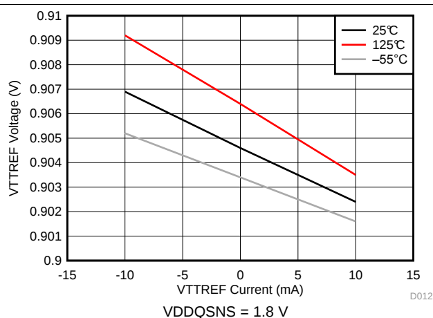
Figure 12. RF Voltage vs REFOUT Current
