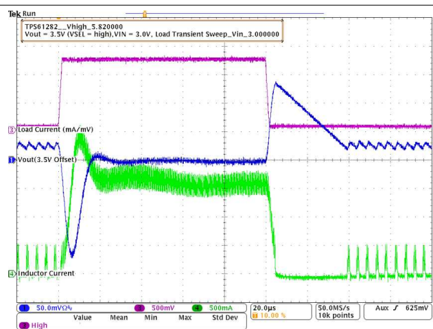
Figure 64. TPS61282A Load Transient Response In PFM/PWM Operation
