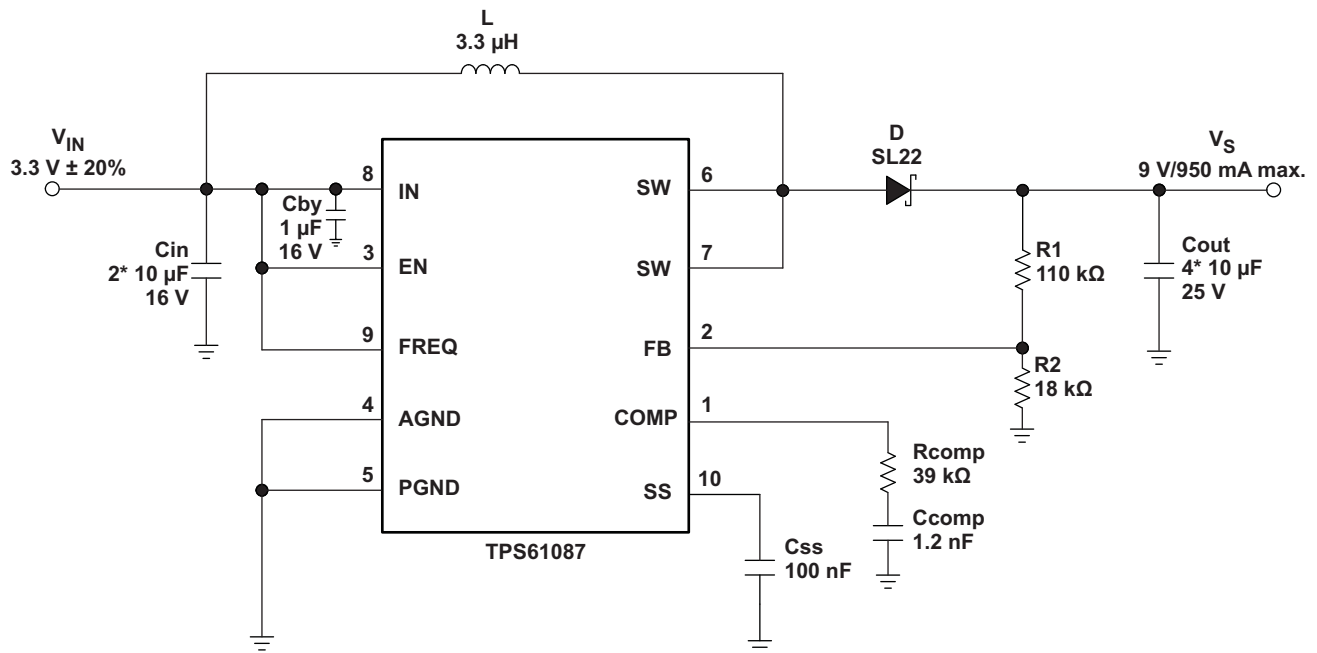
Figure 15. Typical Application, 3.3 V to 9 V ( f_s = 1.2 MHz)
