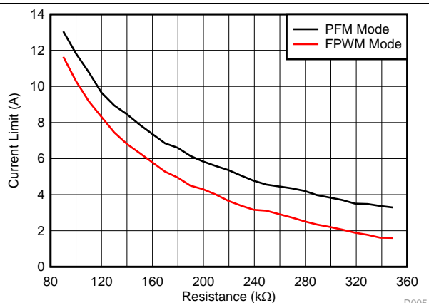
图 5. Current Limit vs Setting Resistance
