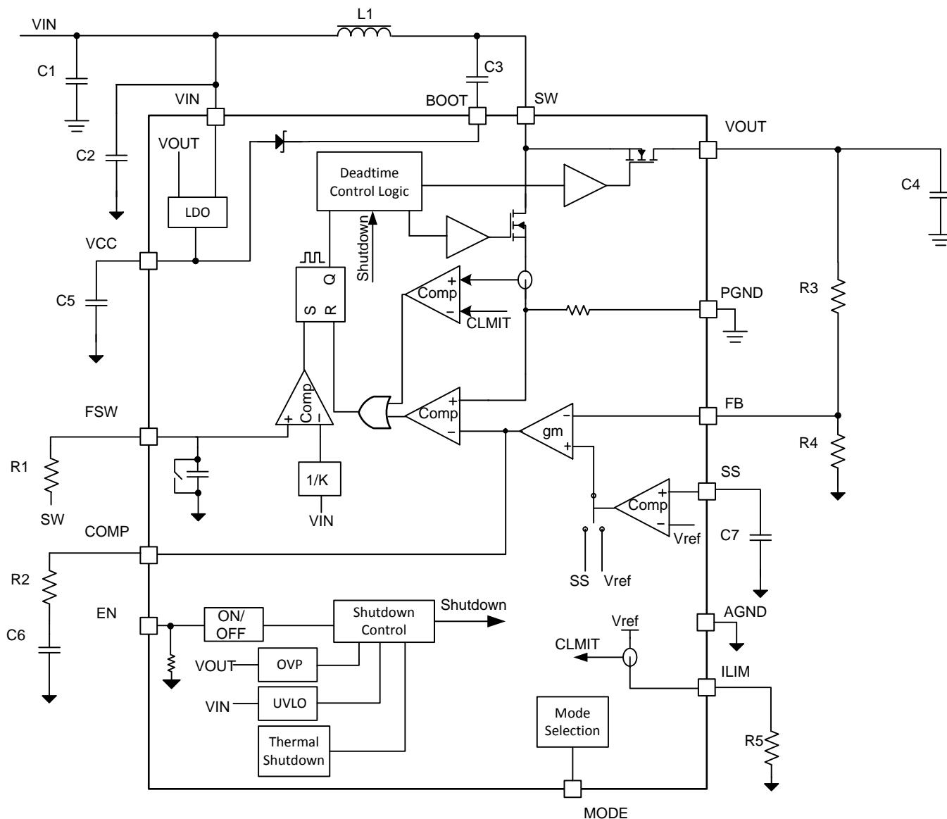
图 10. Functional Block Diagram
