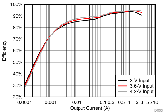
图 1. Efficiency vs Output Current, V_{OUT} = 9\text{ V} , FPWM
