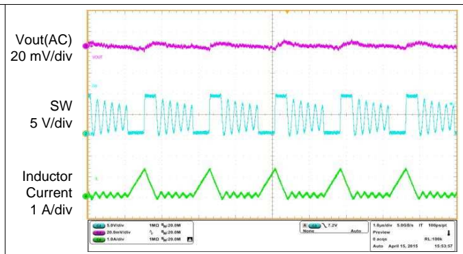
图 14. Switching Waveforms in DCM
