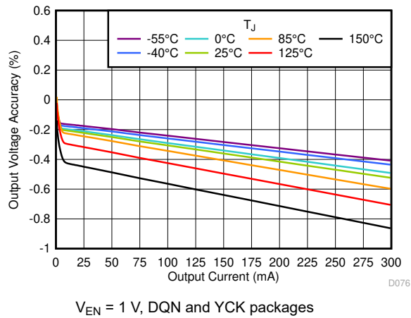
图 6-13. Output Voltage Accuracy vs I_{OUT}
