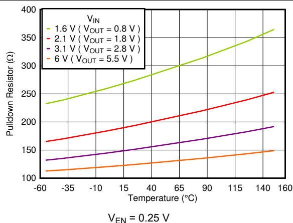
图 6-49. Output Pulldown Resistor vs Temperature
