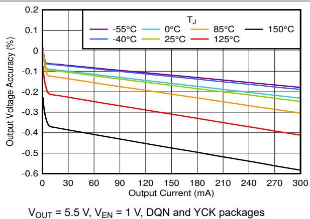
图 6-17. Output Voltage Accuracy vs I_{OUT}
