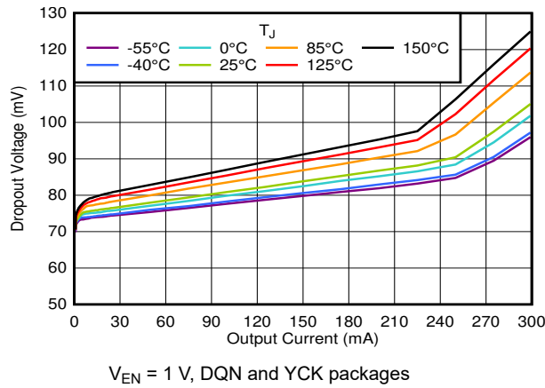
图 6-25. Dropout Voltage vs I_{OUT}
