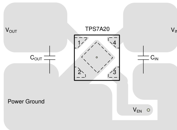
图 10-2. DQN Package (X2SON) Typical Layout
