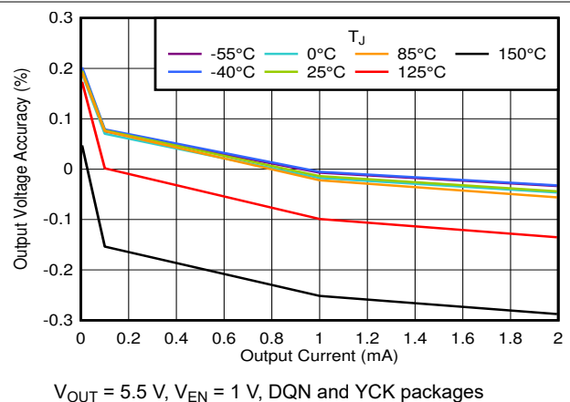
图 6-18. Output Voltage Accuracy vs I_{OUT}
