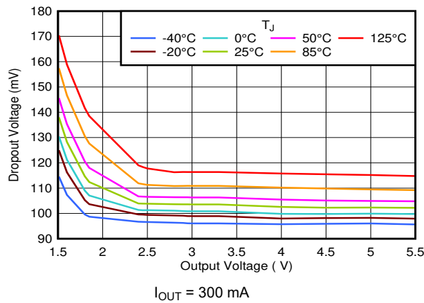
图 6-33. Dropout Voltage vs V_{OUT}
