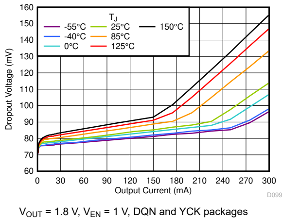
图 6-29. Dropout Voltage vs I_{OUT}
