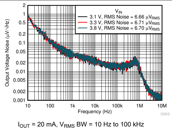
图 6-66. Noise vs Frequency and V_{IN}
