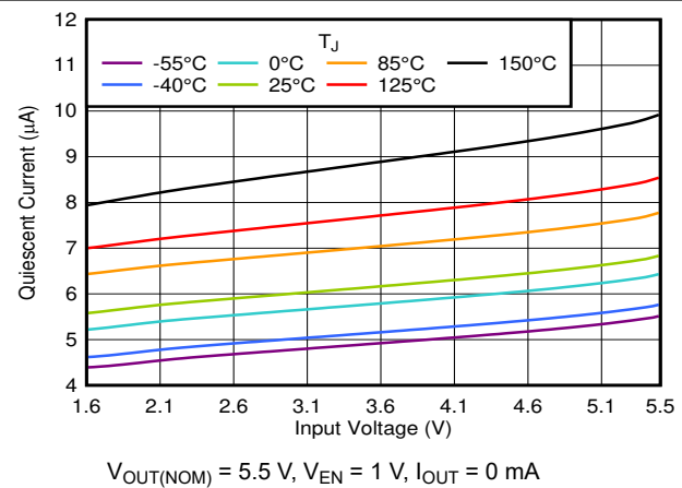
图 6-36. I_{GND} vs V_{IN} in the Dropout Region
