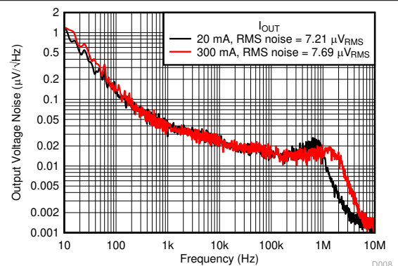
图 6-70. Noise vs Frequency and I_{OUT}
