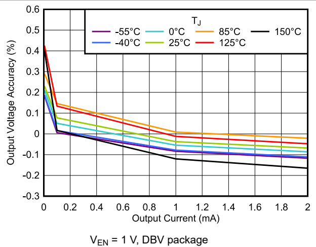
图 6-16. Output Voltage Accuracy vs I_{OUT}
