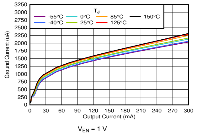
图 6-38. I_{GND} vs I_{OUT}
