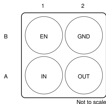
图 5-2. YCK Package (Preview), 4-Pin DSBGA, Bottom View
