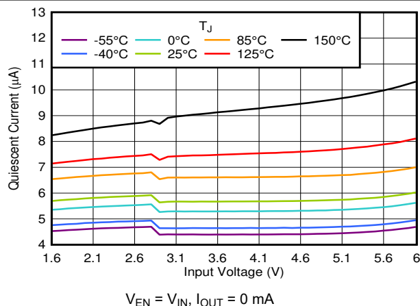
图 6-35. I_{GND} vs V_{IN}
