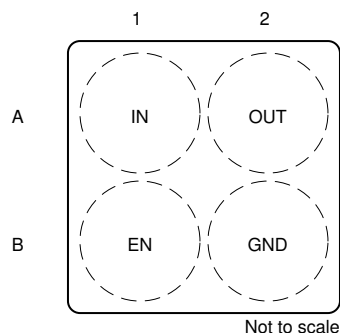
图 5-1. YCK Package (Preview), 4-Pin DSBGA, Top View
