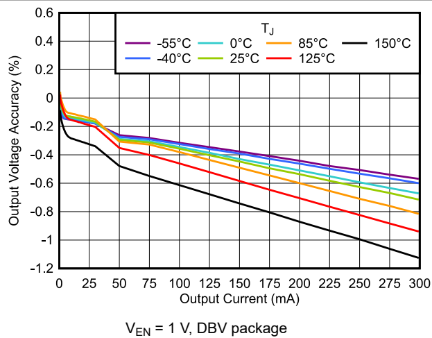
图 6-15. Output Voltage Accuracy vs I_{OUT}
