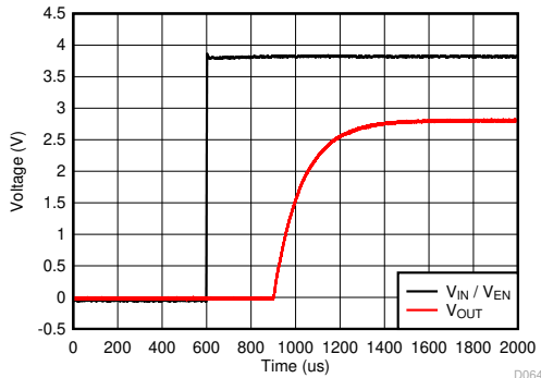
图 8-5. Start-Up
