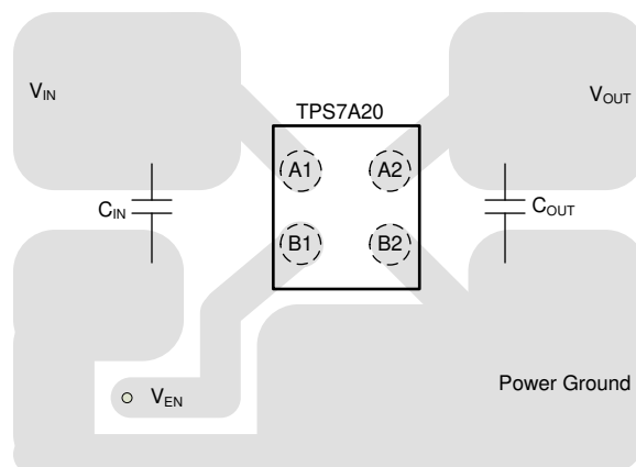
图 10-3. YCK Package (DSBGA) Typical Layout
