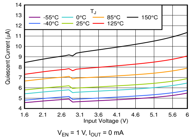
图 6-34. I_{GND} vs V_{IN}
