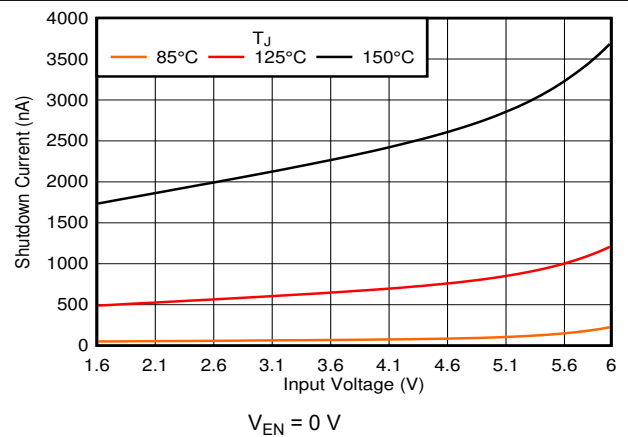
图 6-42. Shutdown Current vs V_{IN}
