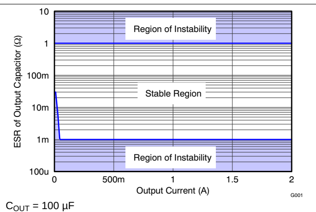
Figure 2. Stability Curve
