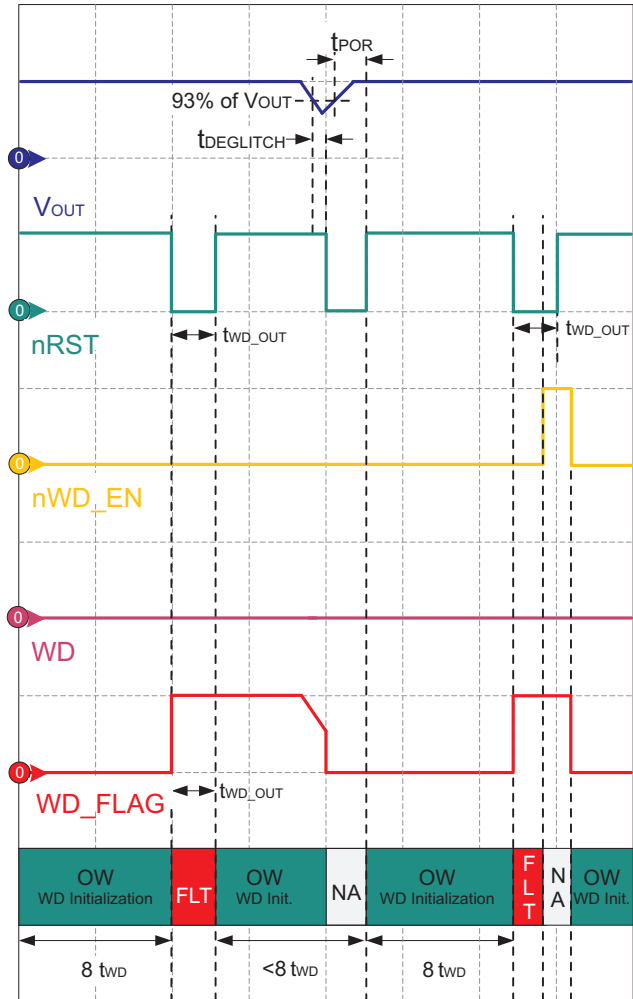
Figure 28. Watchdog Fault During Initialization, and Reinitialization During Reset for TPS7A6401-O1
