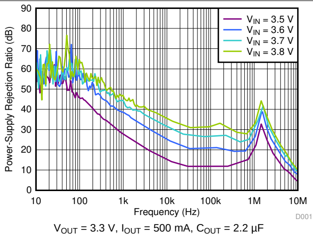
图 25. PSRR vs Frequency and V_{IN}
