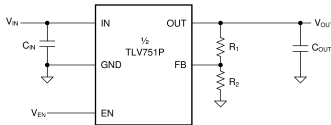
图 38. Adjustable Operation
