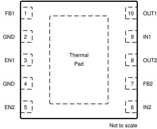
DSQ Package 10-Pin Adjustable WSON Top View
