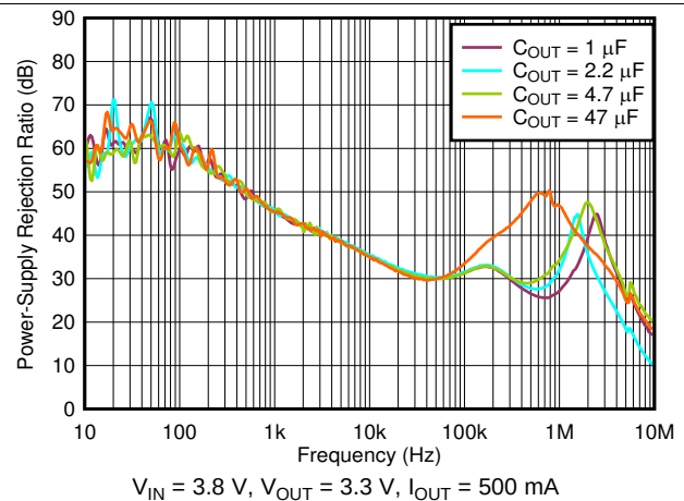
图 30. PSRR vs Frequency and C_{OUT}
