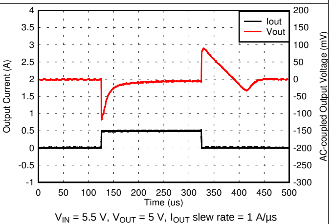
图 22. 5-V, 1-mA to 500-mA Load Transient
