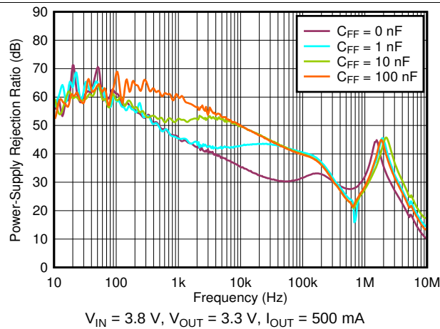
图 31. PSRR vs Frequency and C_{FF}
