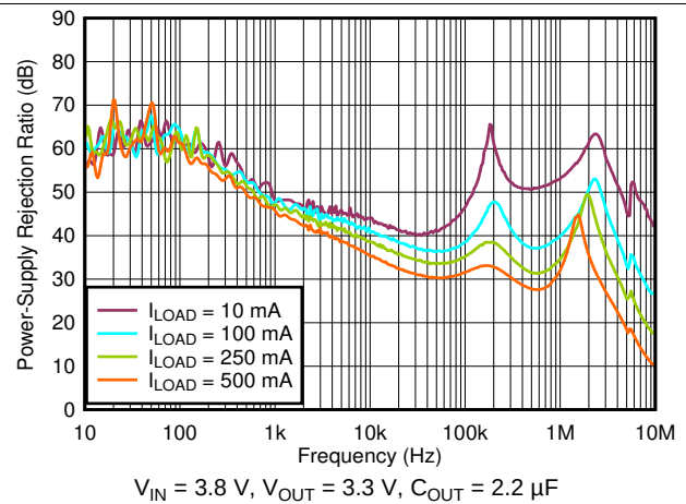
图 32. PSRR vs Frequency and I_{LOAD}
