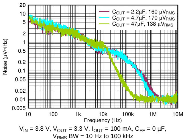
图 35. Output Spectral Noise Density vs Frequency and C_{OUT}
