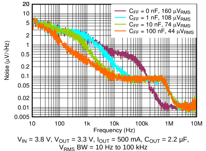
图 34. Output Spectral Noise Density vs Frequency and C_{FF}
