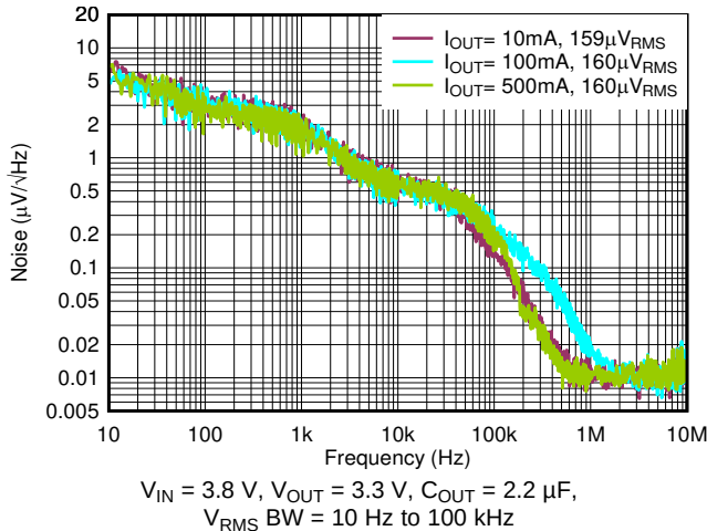
图 33. Output Spectral Noise Density vs Frequency
