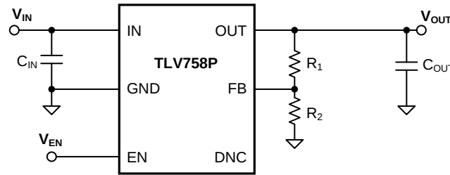
图 42. TLV758P Typical Application
