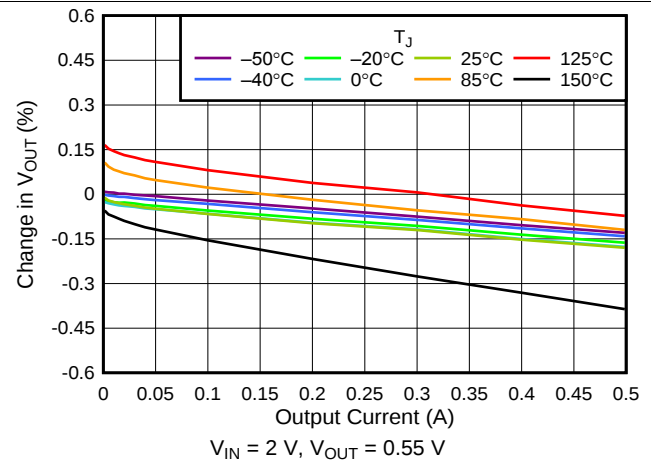
图 12. 0.55-V Load Regulation vs I_{OUT}
