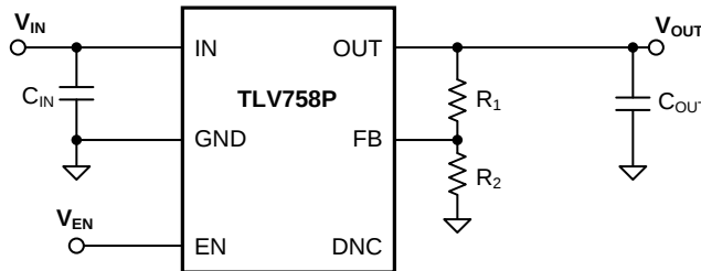
图 38. Adjustable Operation
