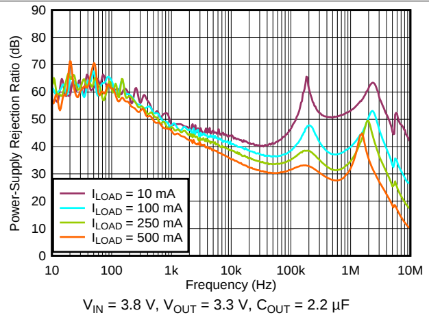
图 32. PSRR vs Frequency and I_{LOAD}
