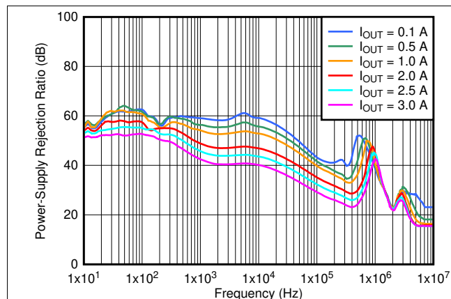
图 10. PSRR vs Frequency and I_{OUT} for V_{OUT} = 5.0 V
