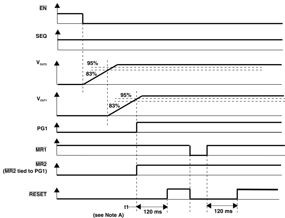
Figure 37. Timing When \overline{MR1} is Toggled
