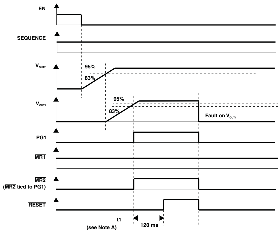
Figure 38. Timing When a Fault Occurs on V_{\text{OUT1}}
