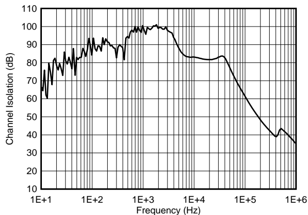
图 45. Channel-to-Channel Isolation
