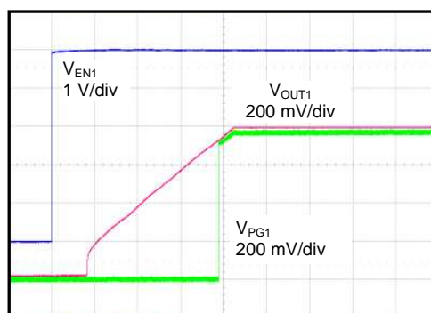
图 20. Start-Up ( SS\_CTRLx = \text{GND} , C_{NR/SSx} = 10\text{ nF} )
