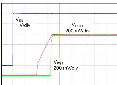
图 19. Start-Up ( SS\_CTRLx = \text{GND} , C_{NR/SSx} = 0\text{ nF} )
