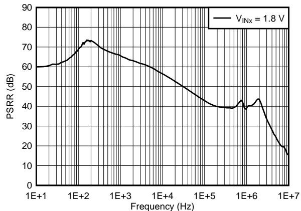
图 44. Power-Supply Rejection
