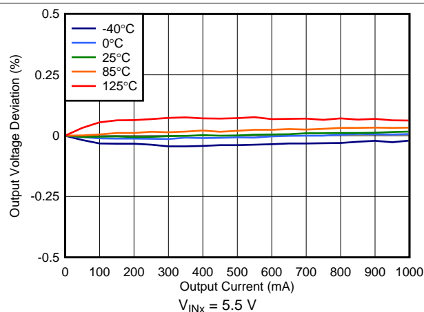
图 29. Load Regulation ( V_{\text{OUTx}} = 5.0\text{ V} )
