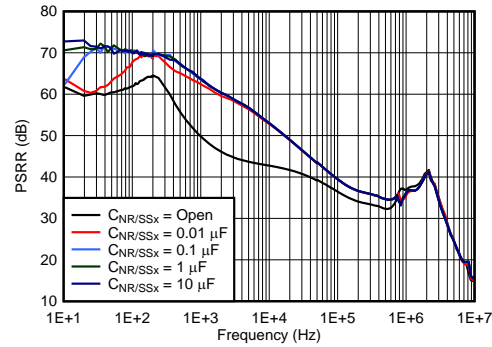
图 2. Power-Supply Rejection vs C_{NR/SSX}
