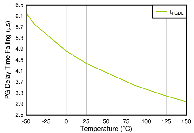
图 6-20. t_{PGDL} vs Temperature
