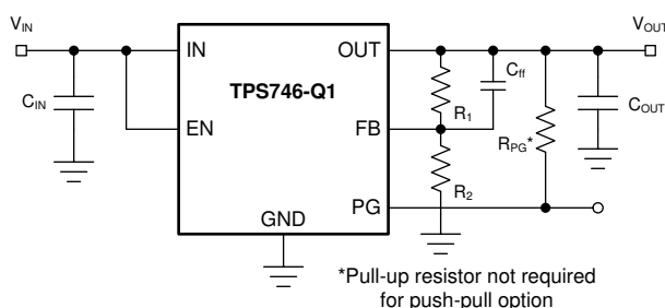
图 8-1. Adjustable Operation
