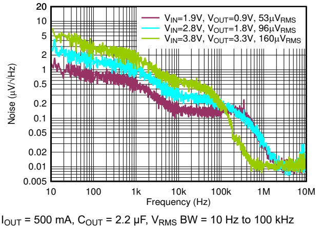
图 6-44. Output Spectral Noise Density vs Frequency
