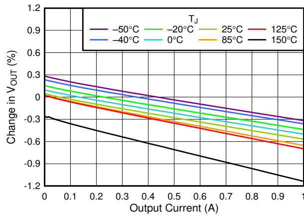
图 6-13. 5-V Load Regulation vs I_{OUT}
