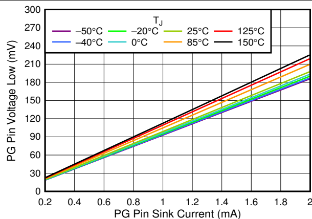
图 6-17. V_{OL}(PG) vs PG Pin Sink Current
