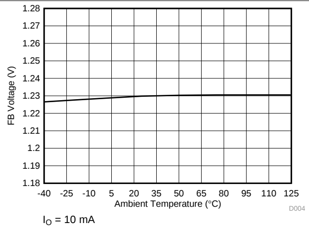
图 6. FB Voltage vs Ambient Temperature
