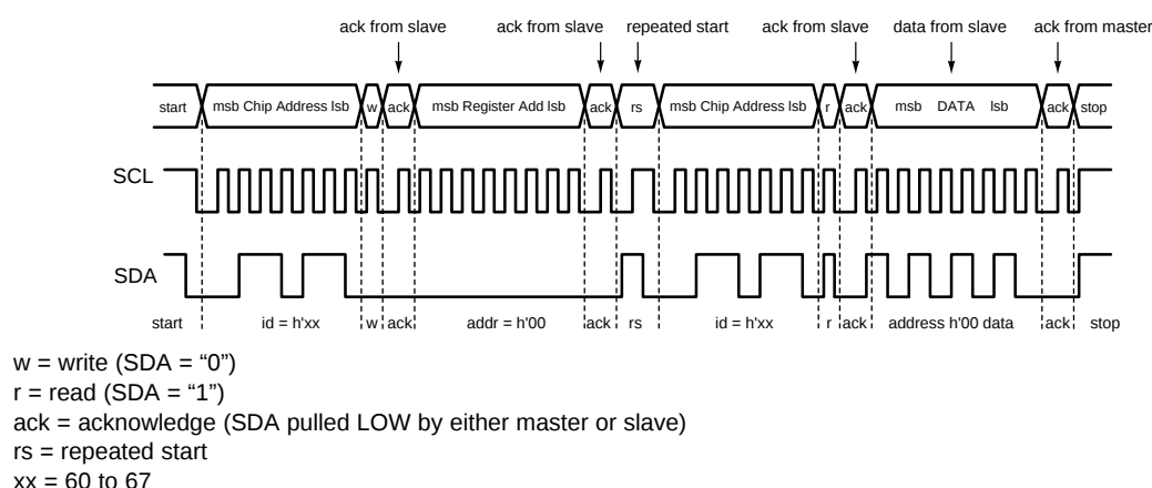
Figure 6. LP3943 Register Read
