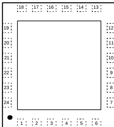
Pin Functions
