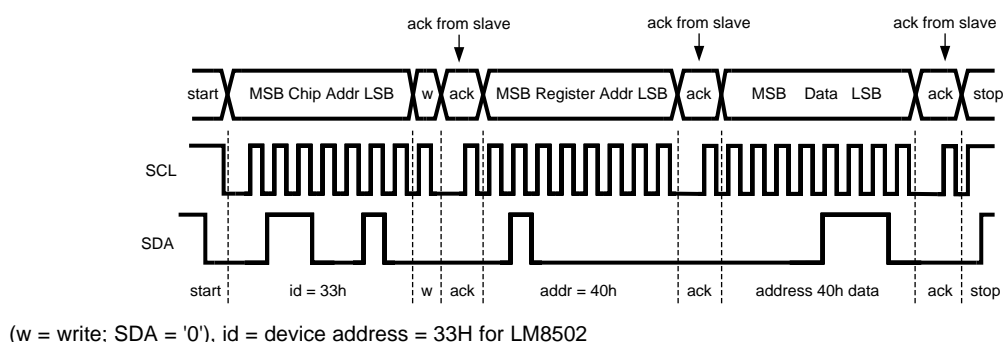
Figure 27. Write Cycle
