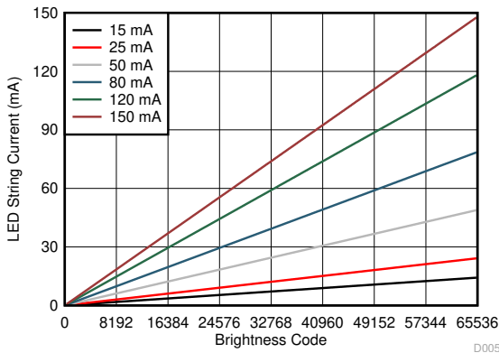
Figure 6-6. Current Linearity
