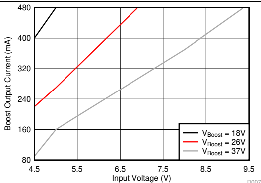
Figure 1. Maximum Boost Current
