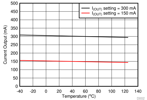
图 3. Output Current vs Temperature
