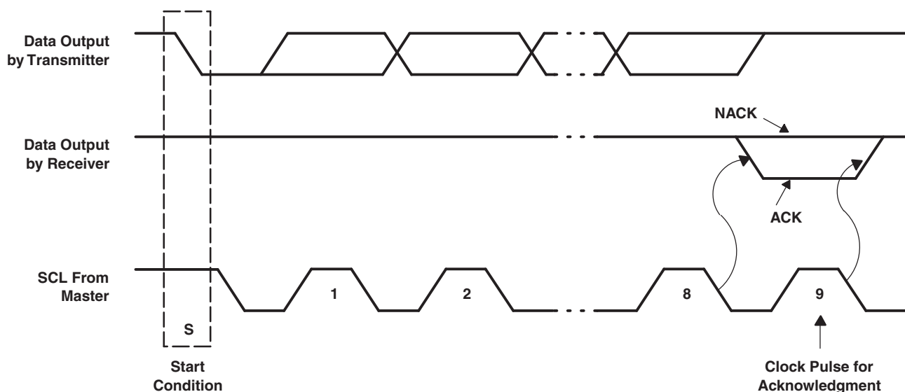
Figure 13. Acknowledge on I²C Bus
