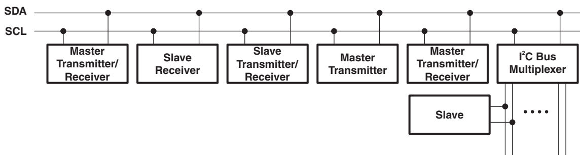
Figure 10. System Configuration
