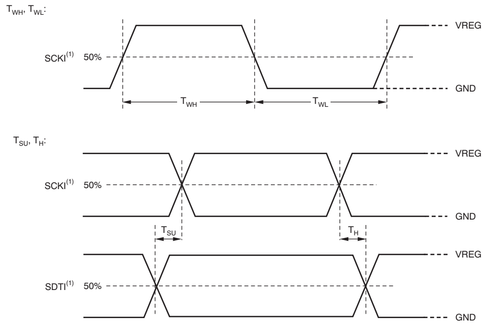
Figure 7. Input Timing
