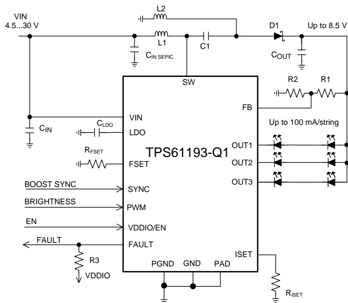
Figure 25. SEPIC Mode, 3 Strings, 100 mA/String Configuration
