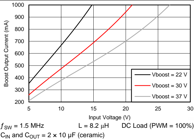
Figure 3. Maximum Boost Current
