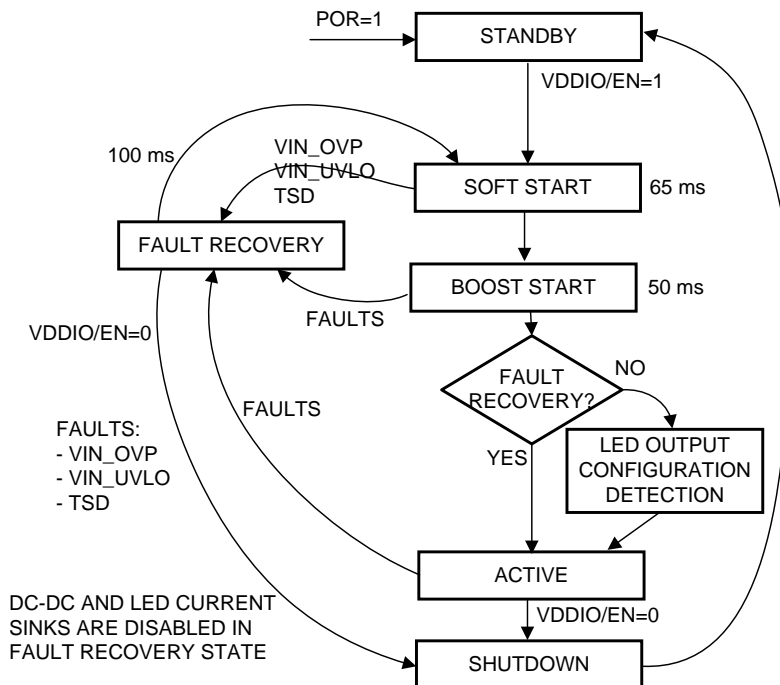
Figure 18. State Diagram
