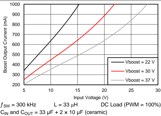
Figure 1. Maximum Boost Current
