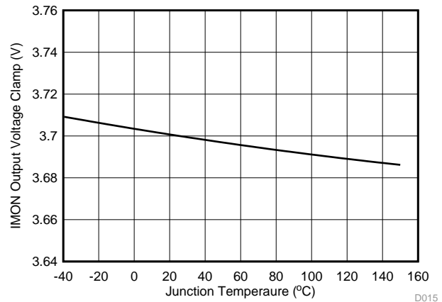
Figure 16. V_{IMON(CLP)} vs Junction Temperature
