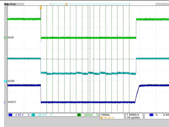
Figure 51. LED Short-Circuit Fault
