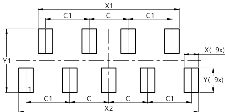
U-DFN3810-9 (Type B)
