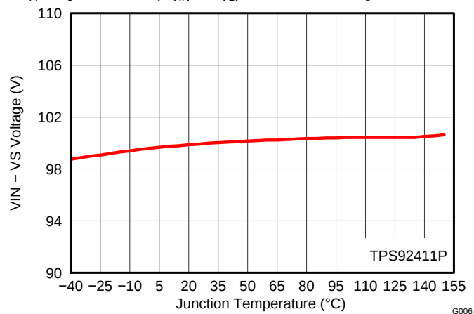
图 7. ( V_{VIN} - V_{VS} ) Overvoltage Threshold vs. Temperature
