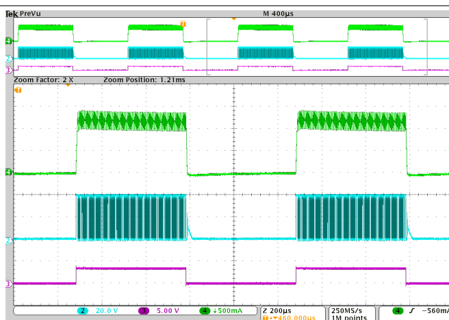
CH4: Inductor Current CH3: PWMx Pin CH2: SWNx Figure 27. PWM Dimming, Two Periods
