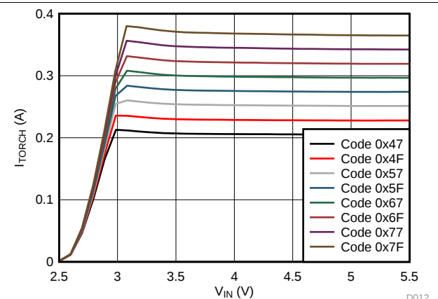
图 11. LED Torch Current vs Input Voltage
