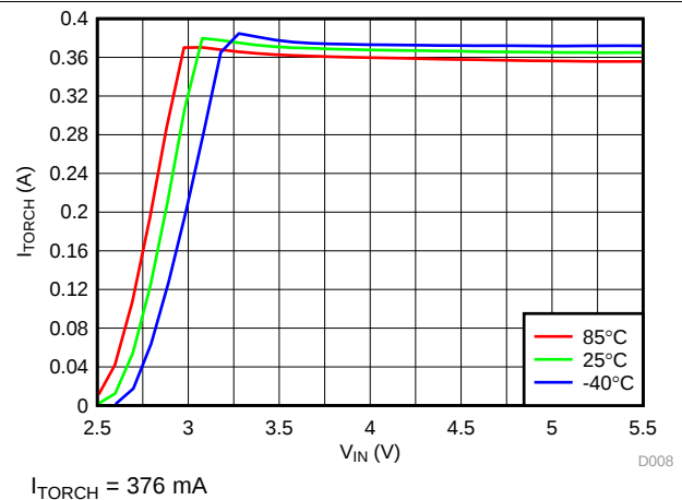
图 9. LED Torch Current vs Input Voltage
