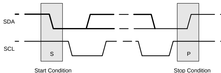
图 21. Start and Stop Conditions
