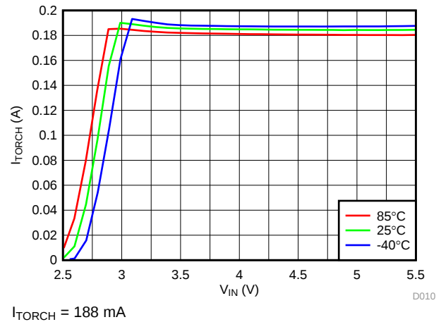
图 11. LED Torch Current vs Input Voltage
