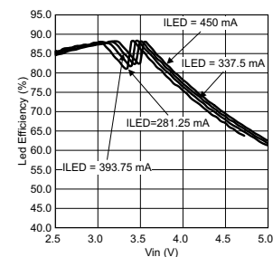
LED 效率与 V_{IN} 双 LED
