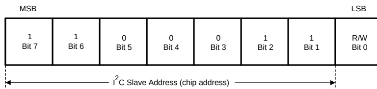
Figure 15. I²C-Compatible Device Address
