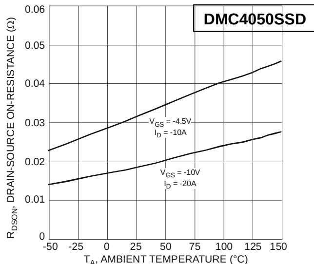
Fig. 18 On-Resistance Variation with Temperature
