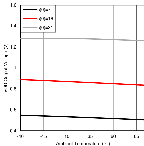
图 2. Typical VOD versus Temperature
