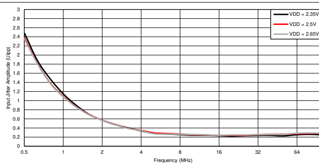
图 6. Typical Input Jitter Tolerance for 30dB channel at 25.78125Gbps for 0.5MHz to 100MHz with Input Random Jitter = 0.078UIpp, T = 25C
