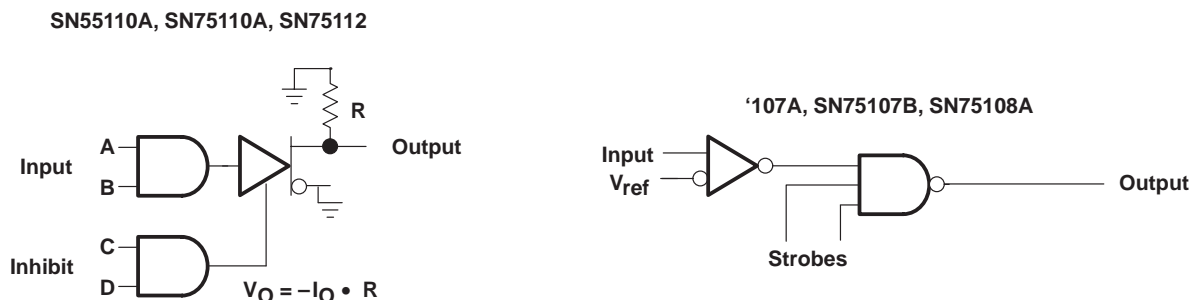
Figure 13. Single-Ended Operation
