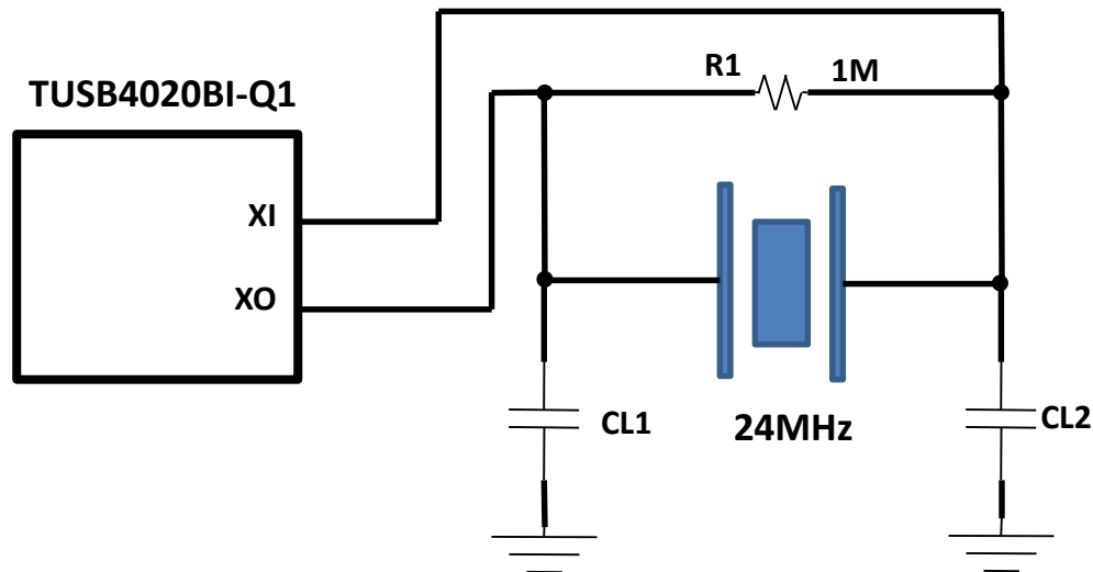
Figure 8-1. TUSB4020BI-Q1 Clock
