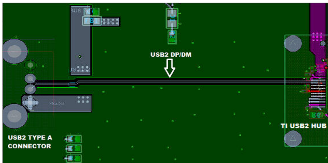
Figure 11-2. Downstream Port
