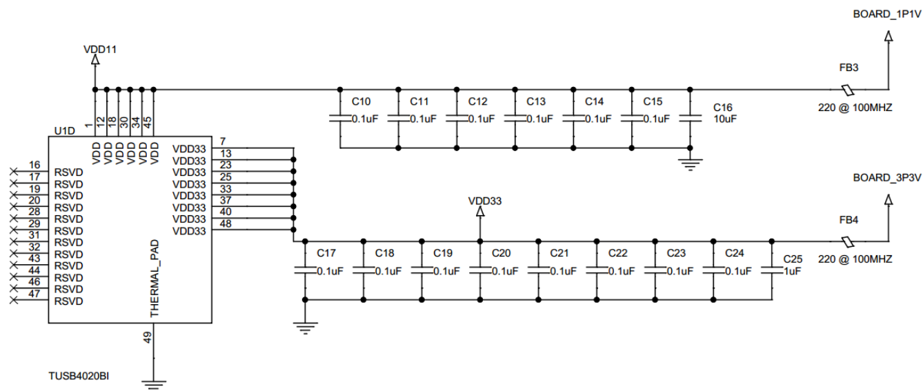
Figure 9-9. Power Implementation Schematic
