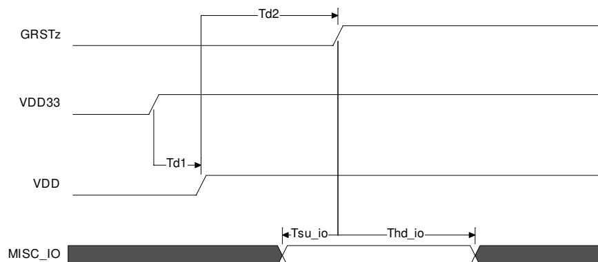
Figure 7-1. Power-Up Timing Requirements
