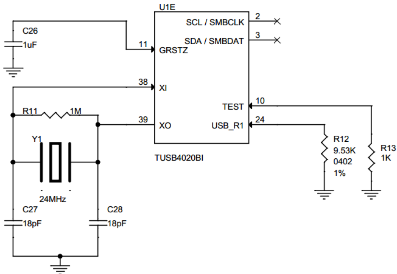
Figure 9-8. Clock, Reset, and Miscellaneous Schematic
