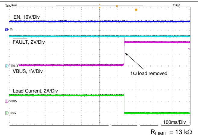
图 98. 1-Ω Load Recovery Without External FET
