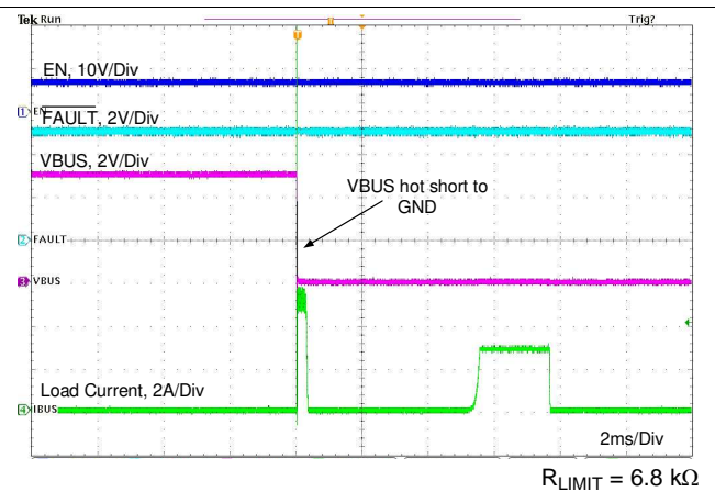
图 102. VBUS Hot Short to GND With External FET
