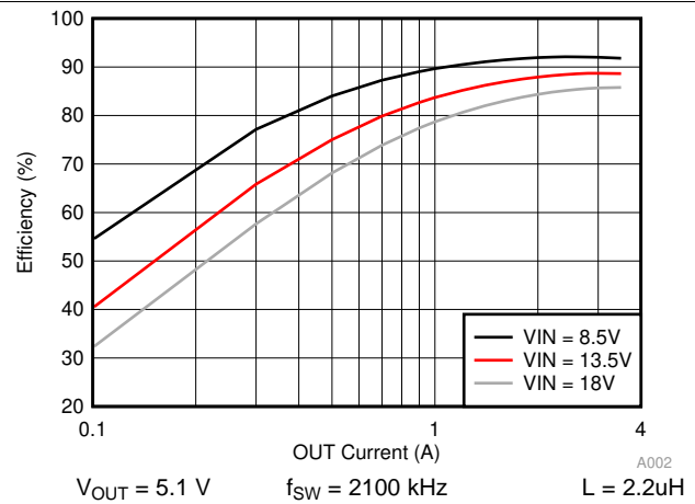
图 76. Buck Only Efficiency
