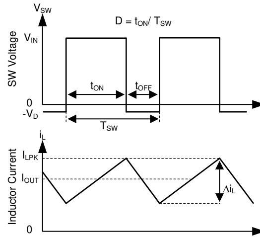
图 39. SW Node and Inductor Current Waveforms in Continuous Conduction Mode (CCM)
