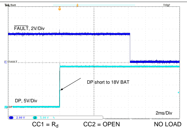
图 108. DP Short to BAT
