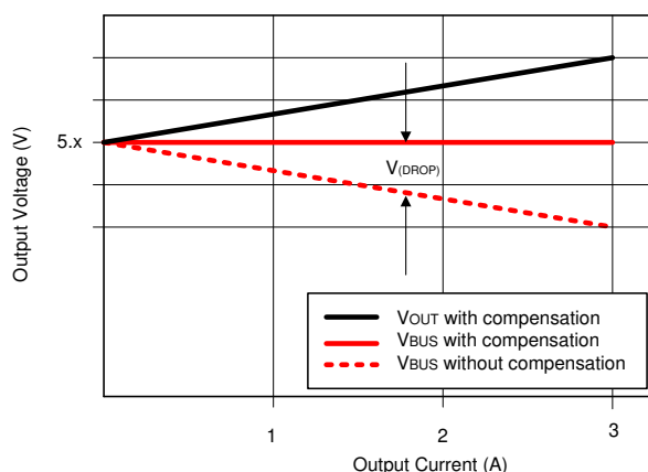
图 61. Voltage Drop
