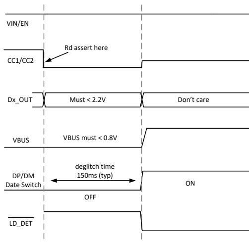
图 43. TPS25830-Q1 Pin Voltage Requirement During Rd Assert
