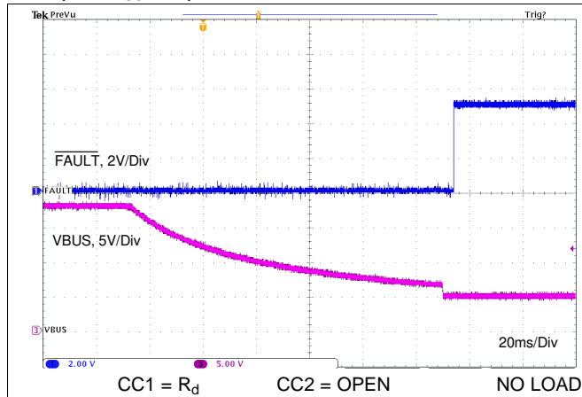
图 105. VBUS Short to BAT Recovery With External FET
