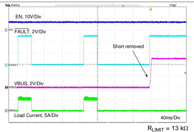
图 96. Short Circuit Recovery Without External FET
