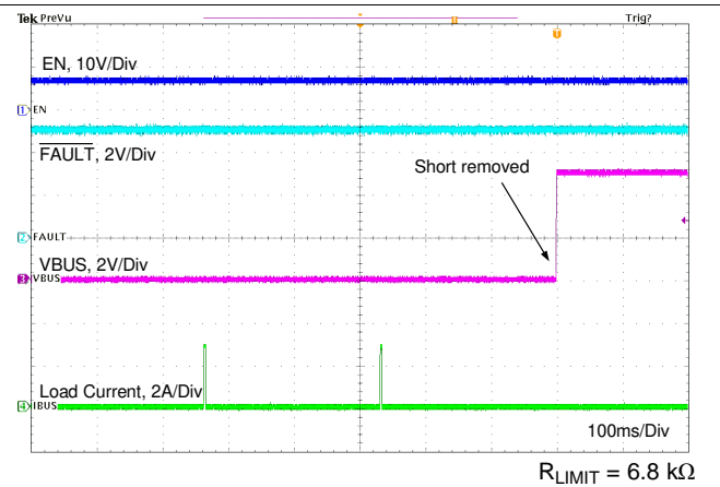
图 100. Short Circuit Recovery With External FET
