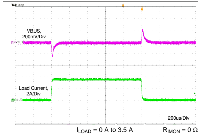
图 81. Load Transient Without Cable Compensation
