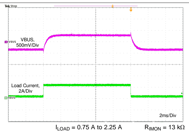
图 84. Load Transient With Cable Compensation
