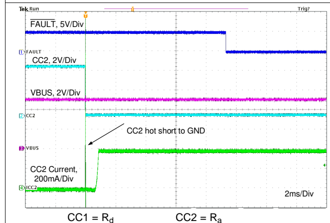
图 103. CC2 Hot Short to GND
