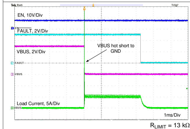
图 101. VBUS Hot Short to GND Without External FET
