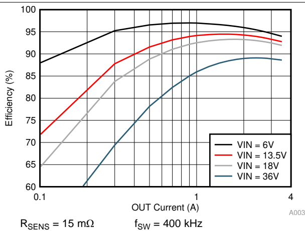
图 77. Efficiency With Sense Resistor
