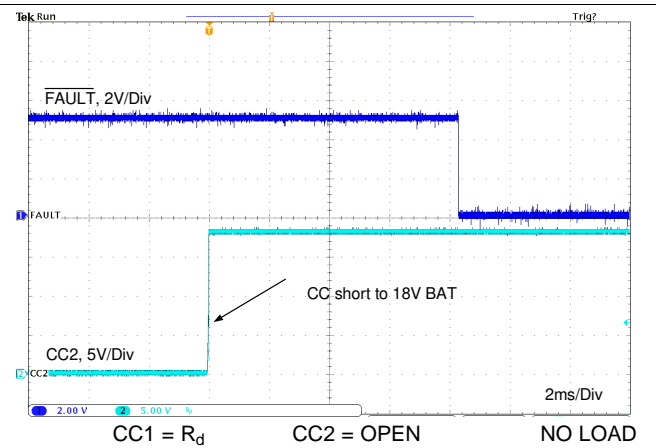
图 106. CC Short to BAT
