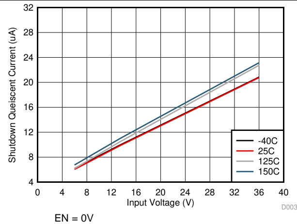
图 3. Shutdown Quiescent Current
