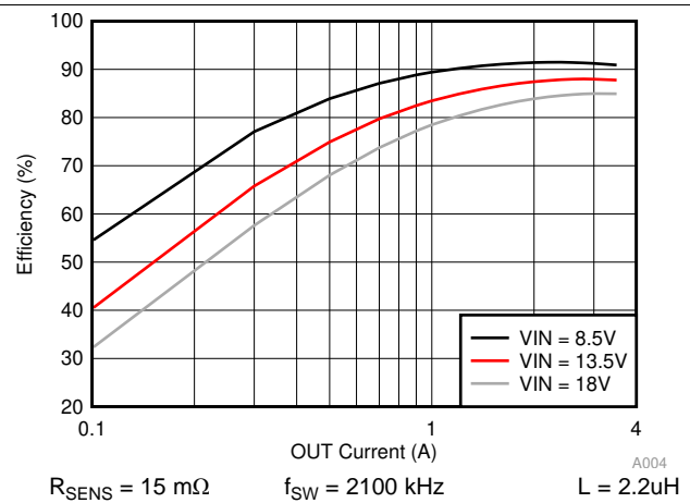
图 78. Efficiency With Sense Resistor
