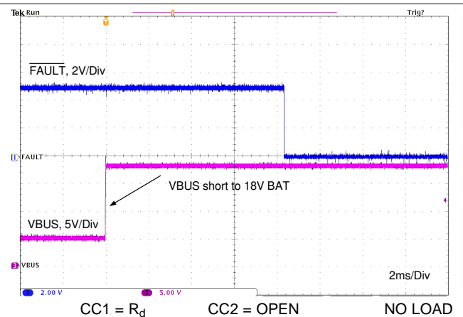
图 104. VBUS Short to BAT With External FET
