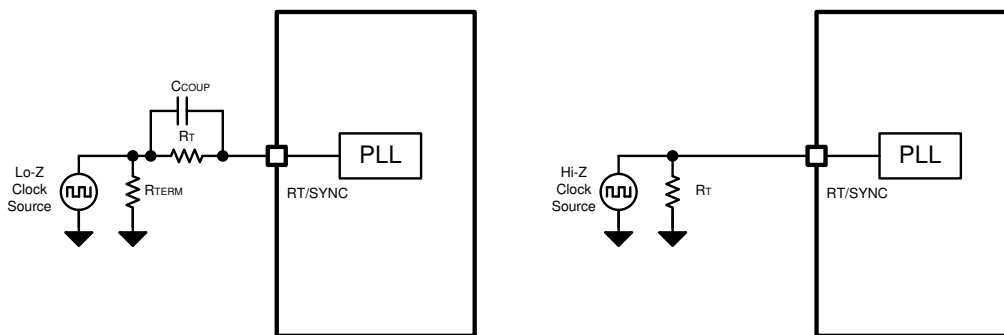
图 45. Synchronize to External Clock
