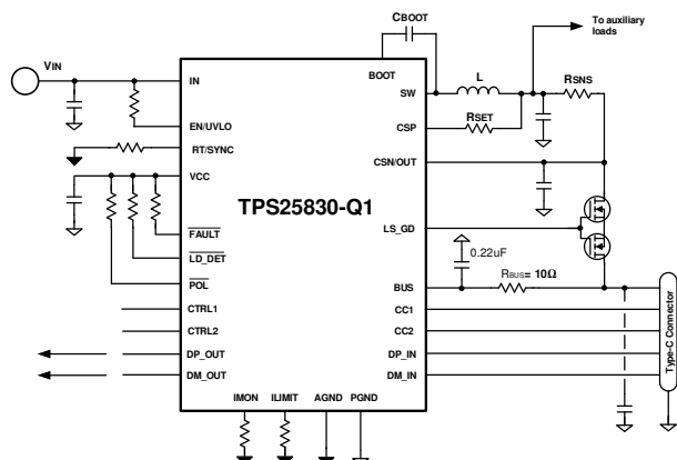
图 58. Current Limit With External MOSFET
