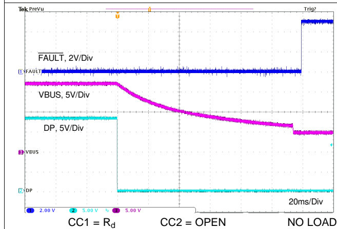
图 109. DP Short to BAT Recovery
