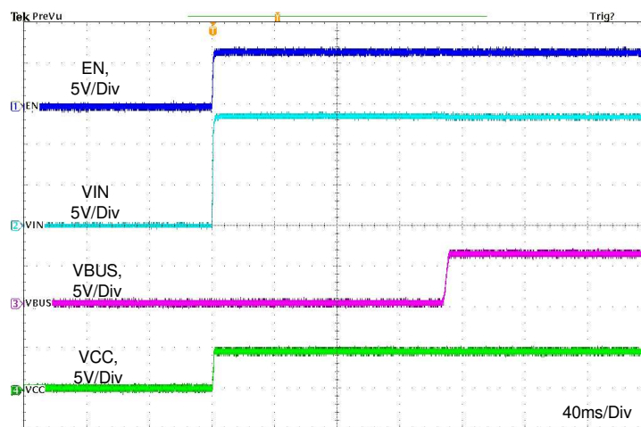
图 42. Typical Start-up Behavior, V_{IN} = 13.5 \text{ V} , CC1 = R_d , R_{IMON} = 12.6 \text{ k}\Omega
