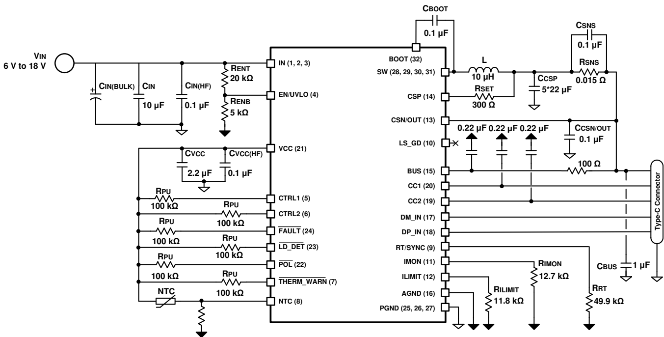
图 74. Application Circuit
