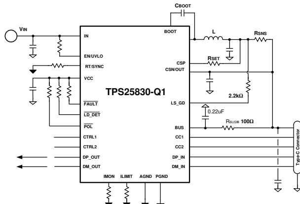
图 59. Buck Average Current Limit
