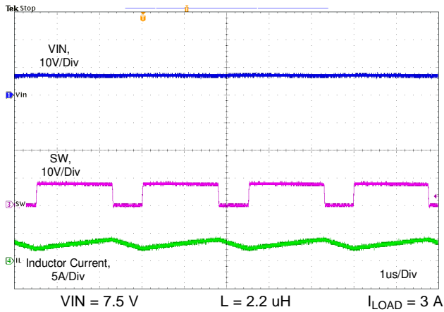
图 46. Switching Frequency When R_T = 8.87 \text{ k}\Omega
