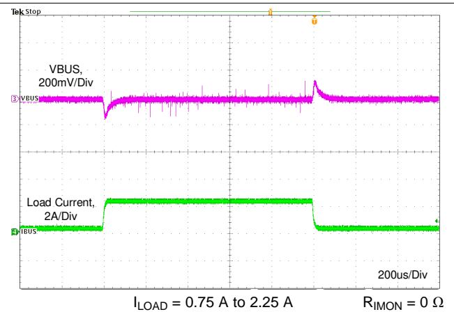
图 82. Load Transient Without Cable Compensation
