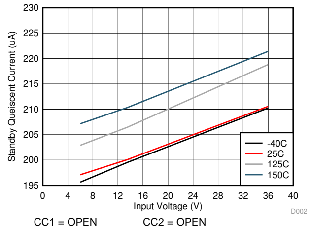
图 2. Standby Quiescent Current
