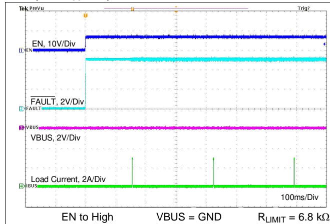
图 99. Enable Into Short With External FET
