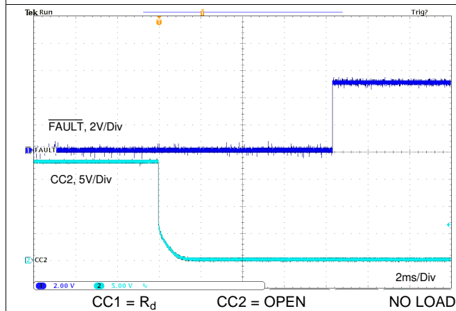
图 107. CC Short to BAT Recovery
