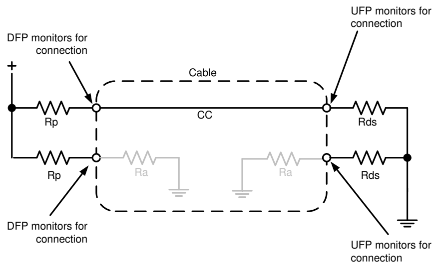
图 63. DFP-UFP Connection
