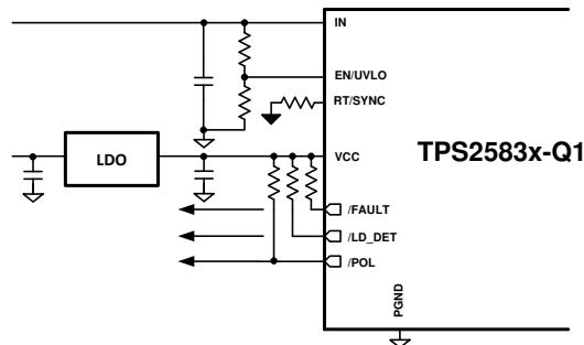
图 52. V CONN Source Using External LDO
