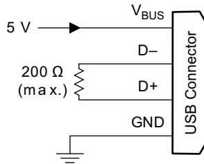
图 70. DCP Supporting BC1.2 and YD/T 1591-2009
