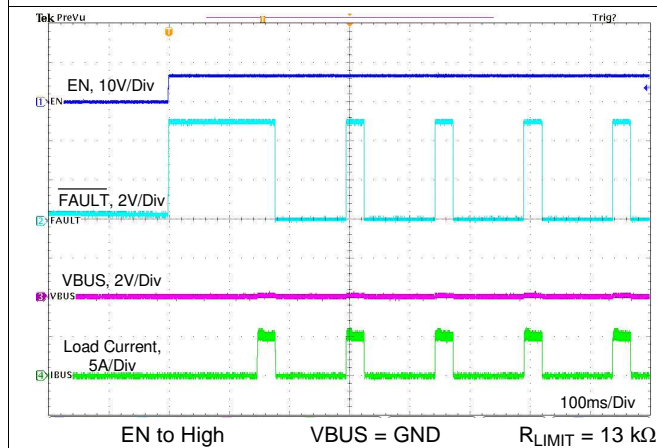
图 95. Enable Into Short Without External FET
