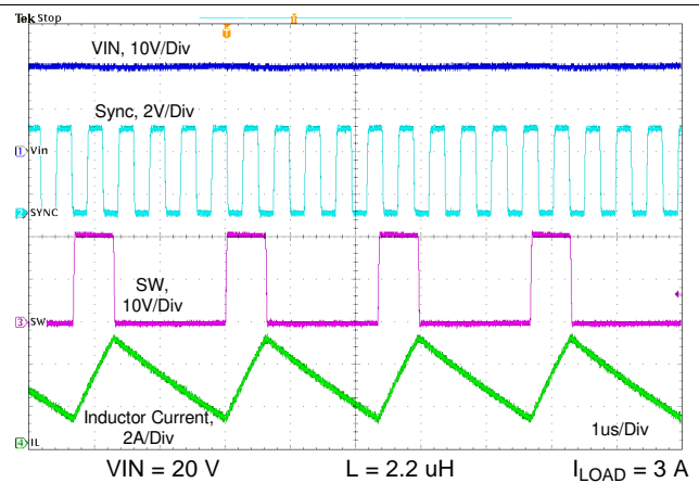
图 51. Synchronizing to External 2.1-MHz Clock
