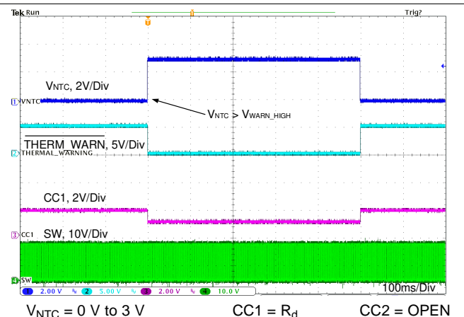
图 110. Thermal Sensing With NTC Behavior 1
