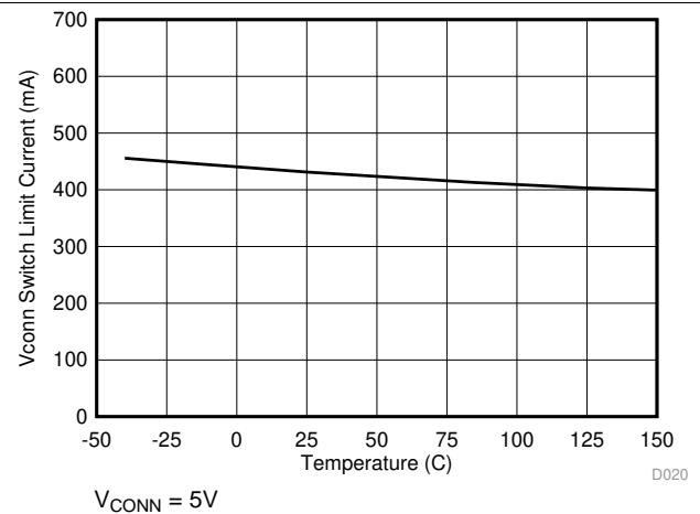
图 24. V CONN Switch Current Limit vs Junction Temperature
