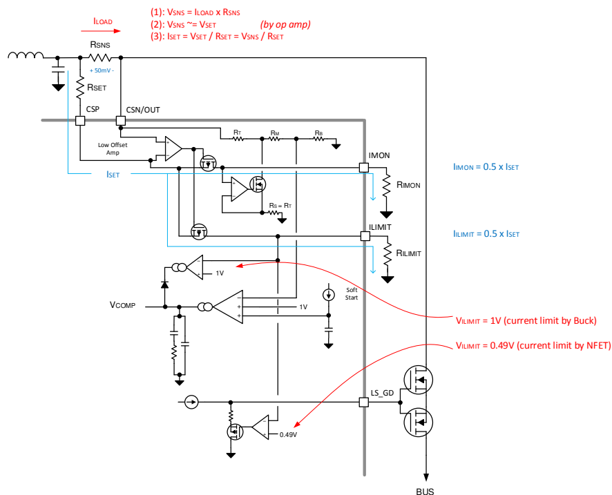
图 53. Current Limit and Cable Compensation Circuit
