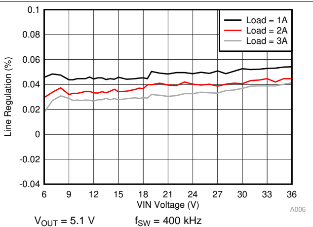
图 80. Line Regulation
