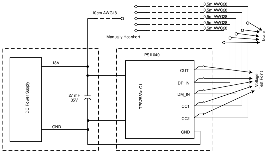
图 38. Short-to-Battery System Test Setup
