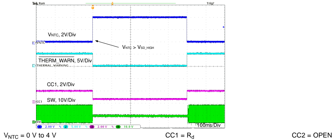
图 111. Thermal Sensing With NTC Behavior 2
