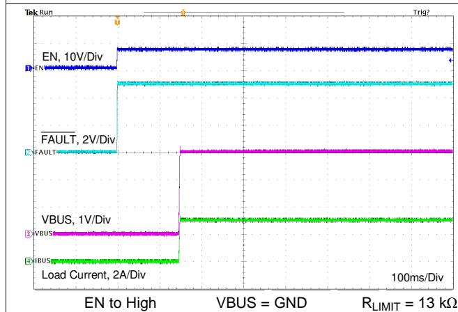
图 97. Enable Into 1-Ω Load Without External FET
