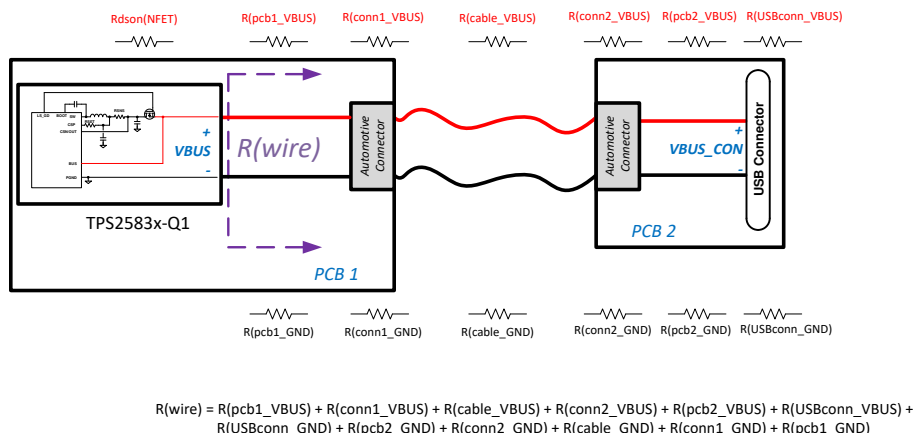
图 60. Automotive USB Resistances
