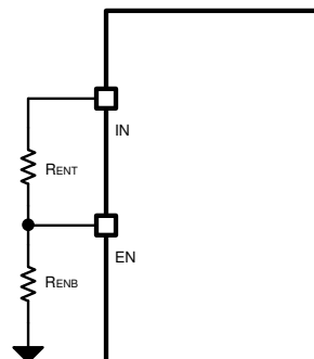
图 41. System UVLO by Enable Divider
