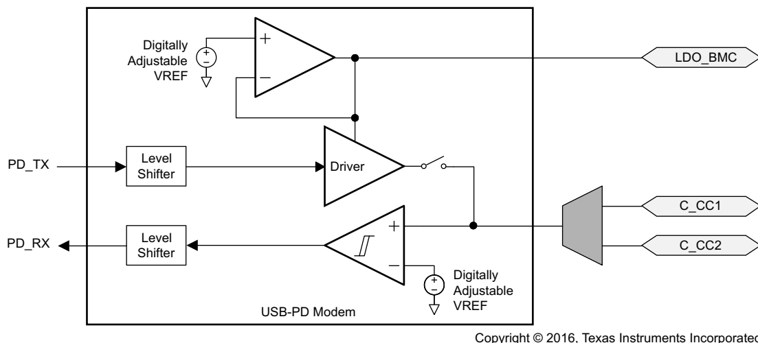
Figure 14. USB-PD BMC TX/Rx Block Diagram
