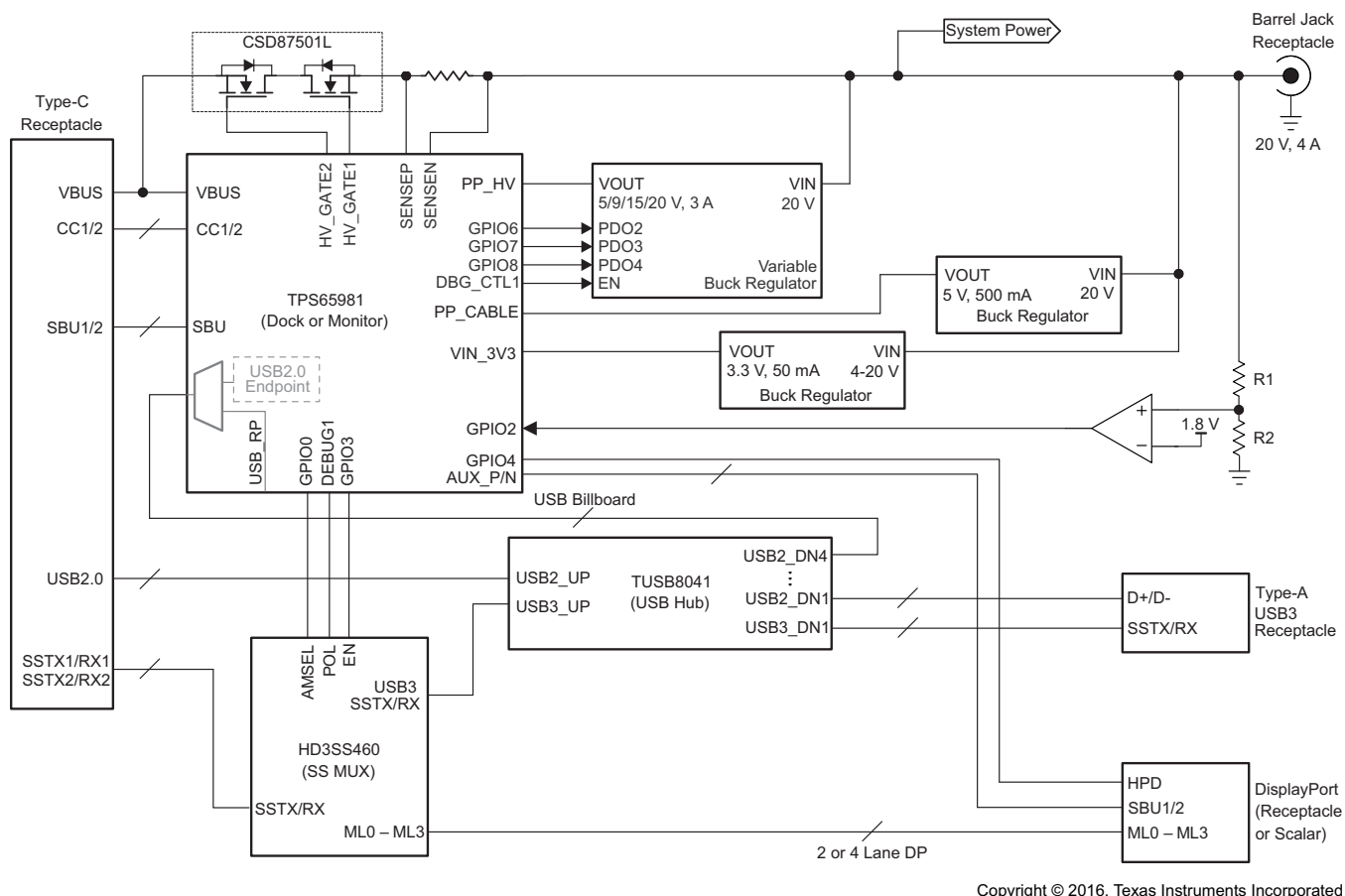
Figure 76. Type-C and PD Dock or Monitor Application
