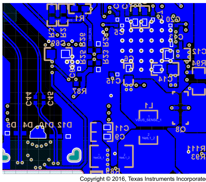
Figure 91. Bottom Layer Component Routing
