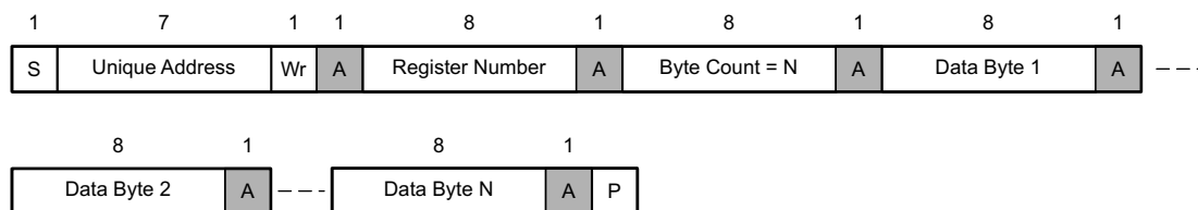
Figure 70. I²C Unique Address Write Register Protocol
