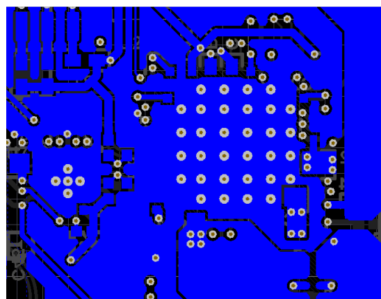
Figure 94. Final Routing (Bottom Layer)
