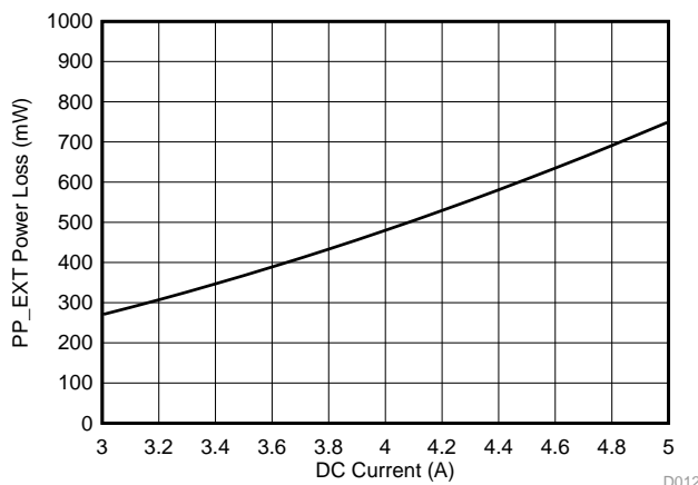
Figure 75. PP_EXT Power Loss ( R_{NFETS} + R_{SENSE} = 30\text{ m}\Omega )
