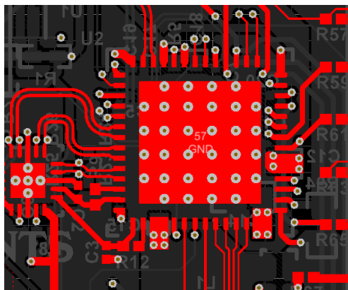
Figure 92. Final Routing (Top Layer)
