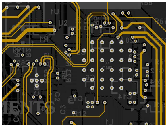
Figure 93. Final Routing (Inner Signal Layer)
