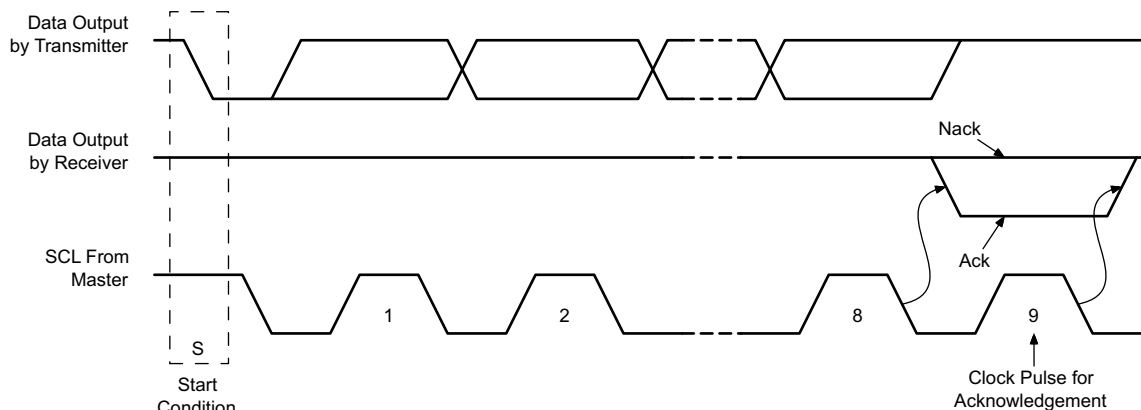
Figure 69. I²C Acknowledgment
