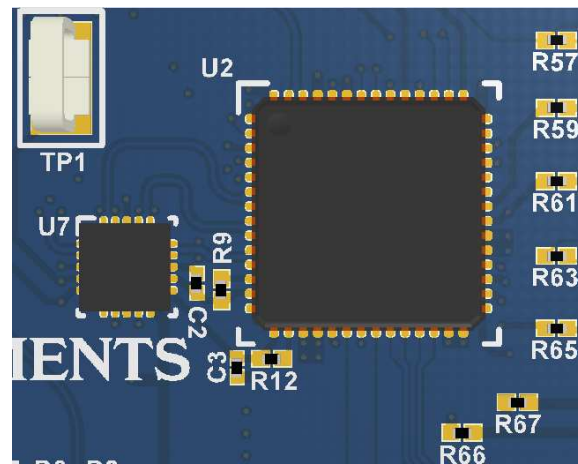
Figure 85. Example Layout (Top View in 3-D)
