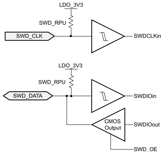
Figure 60. IOBUF_GPIOHSSWD
