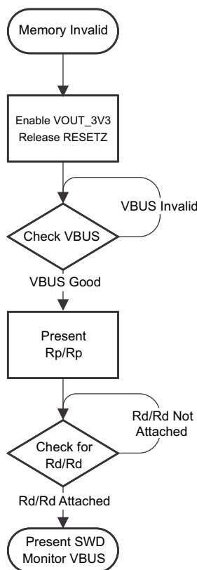
Figure 66. Memory Invalid Flow
