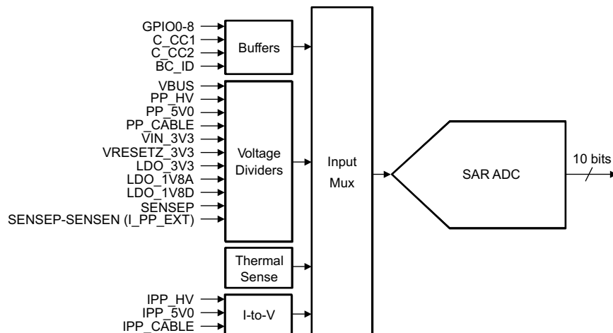
Figure 53. SAR ADC
