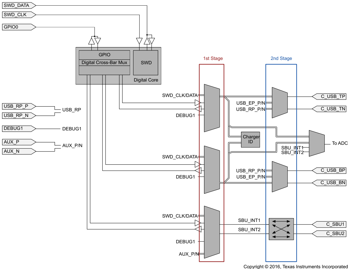
Figure 44. Port Data Multiplexers
