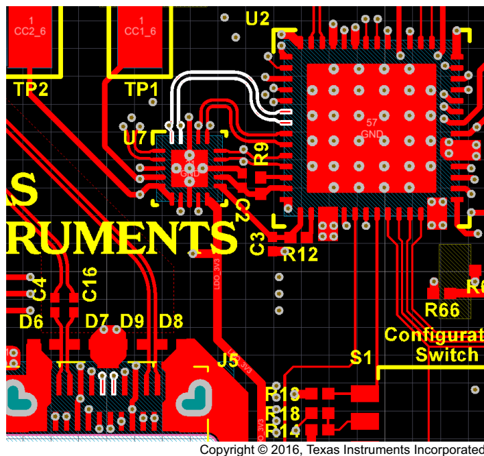
Figure 90. Top Layer Component Routing
